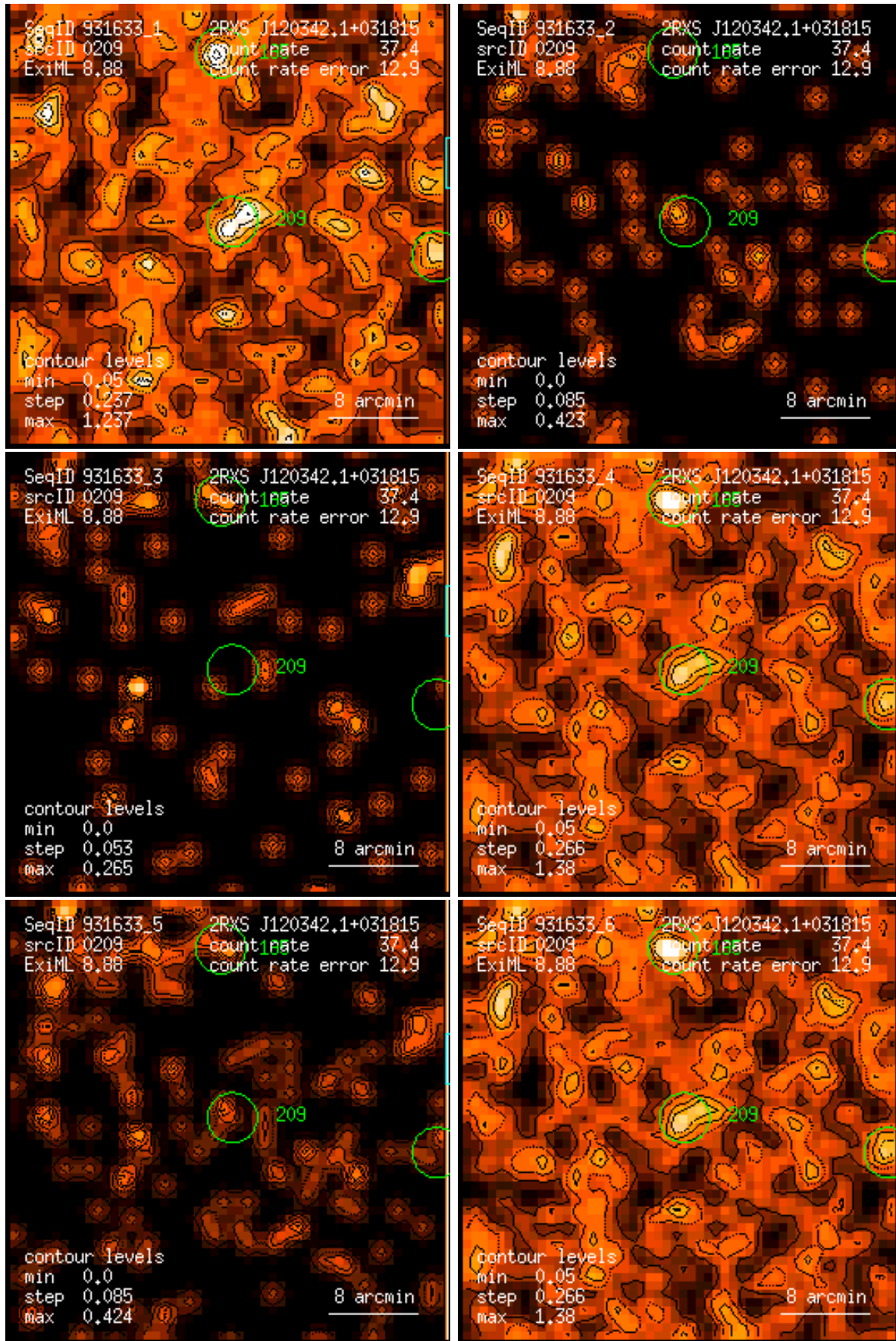
Figure 209: RASS 931633: detection 0209: band rate images, Gaussian filter: (1) PSPC channels 11 – 41, (2) 52 – 90, (3) 91 – 201, (4) 11 – 235, (5) 52 – 201, (6) 11 – 201. Broad band rates in counts/ks. Band rate contour levels in counts/ks/arcmin 2 .
