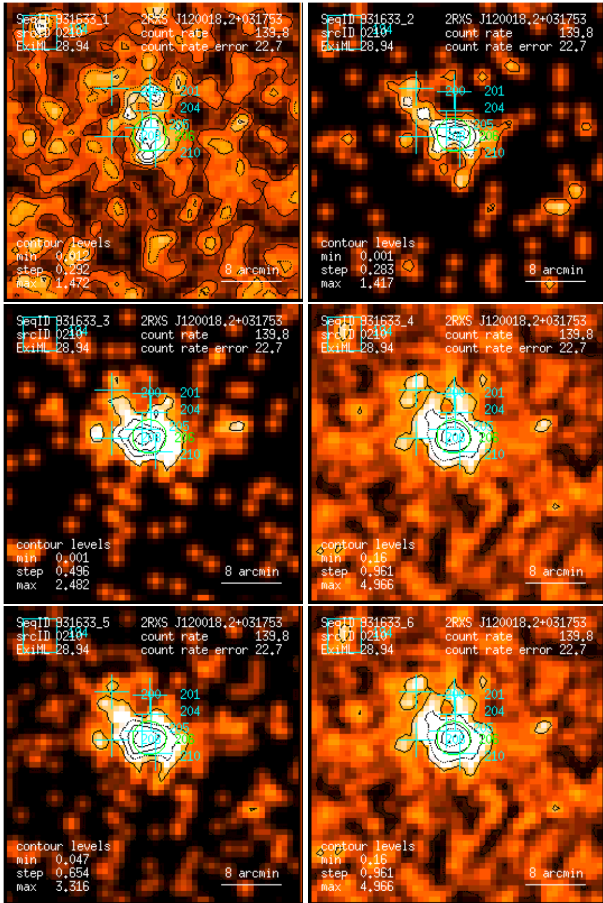
Figure 210: RASS 931633: detection 0210: band rate images, Gaussian filter: (1) PSPC channels 11 – 41, (2) 52 – 90, (3) 91 – 201, (4) 11 – 235, (5) 52 – 201, (6) 11 – 201. Broad band rates in counts/ks. Band rate contour levels in counts/ks/arcmin 2 .
