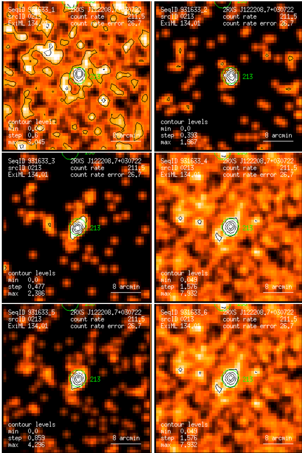
Figure 213: RASS 931633: detection 0213: band rate images, Gaussian filter: (1) PSPC channels 11 – 41, (2) 52 – 90, (3) 91 – 201, (4) 11 – 235, (5) 52 – 201, (6) 11 – 201. Broad band rates in counts/ks. Band rate contour levels in counts/ks/arcmin 2 .
