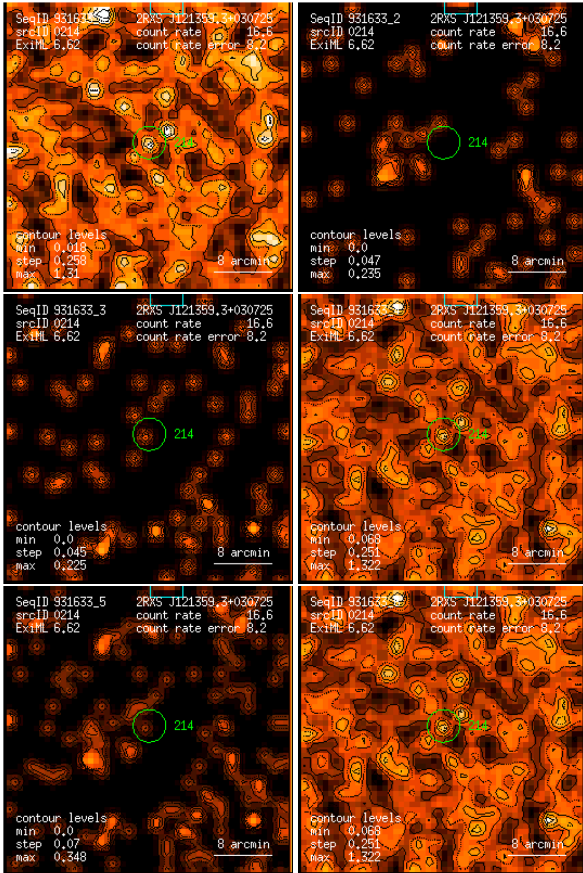
Figure 214: RASS 931633: detection 0214: band rate images, Gaussian filter: (1) PSPC channels 11 – 41, (2) 52 – 90, (3) 91 – 201, (4) 11 – 235, (5) 52 – 201, (6) 11 – 201. Broad band rates in counts/ks. Band rate contour levels in counts/ks/arcmin 2 .
