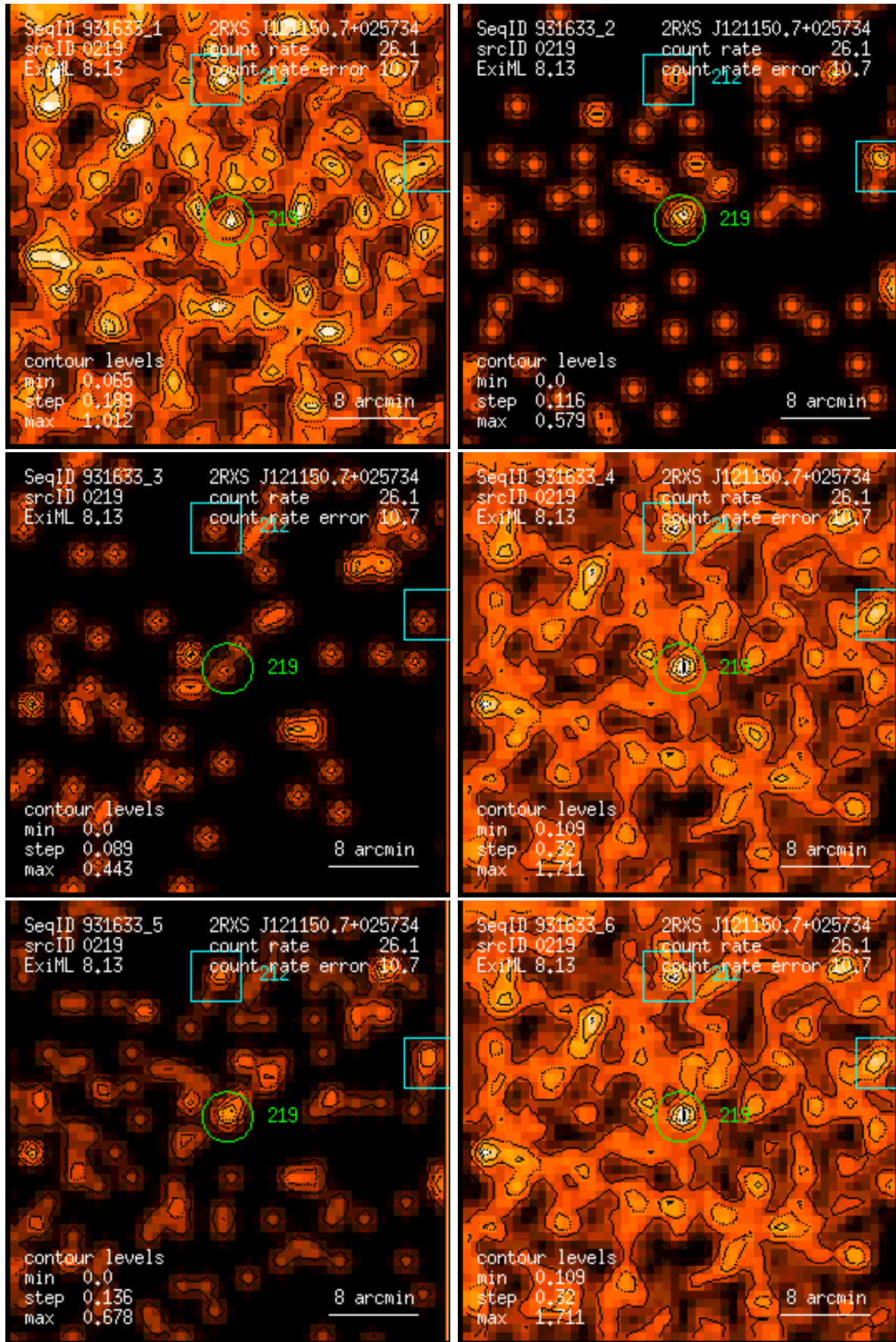
Figure 219: RASS 931633: detection 0219: band rate images, Gaussian filter: (1) PSPC channels 11 – 41, (2) 52 – 90, (3) 91 – 201, (4) 11 – 235, (5) 52 – 201, (6) 11 – 201. Broad band rates in counts/ks. Band rate contour levels in counts/ks/arcmin 2 .
