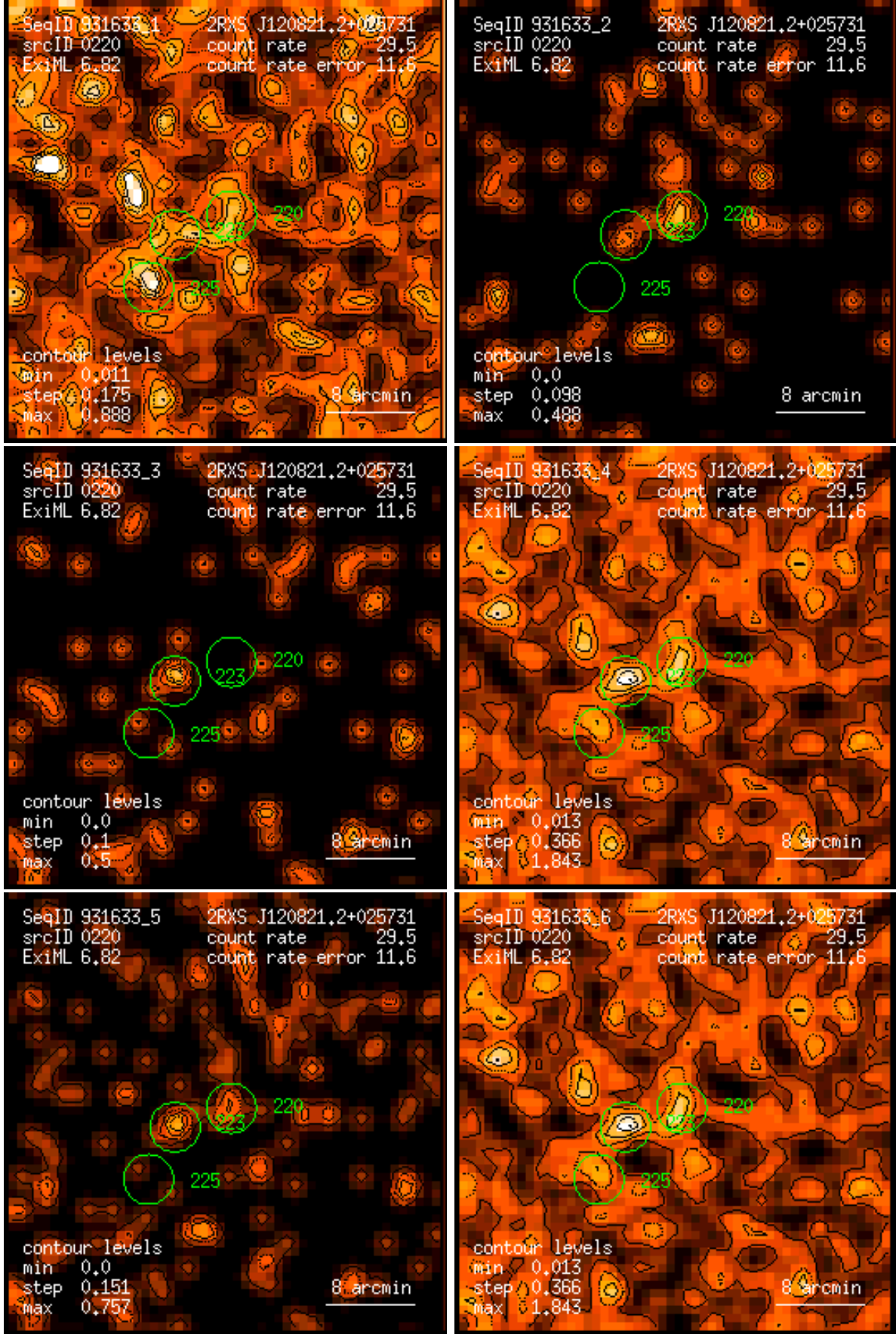
Figure 220: RASS 931633: detection 0220: band rate images, Gaussian filter: (1) PSPC channels 11 – 41, (2) 52 – 90, (3) 91 – 201, (4) 11 – 235, (5) 52 – 201, (6) 11 – 201. Broad band rates in counts/ks. Band rate contour levels in counts/ks/arcmin 2 .
