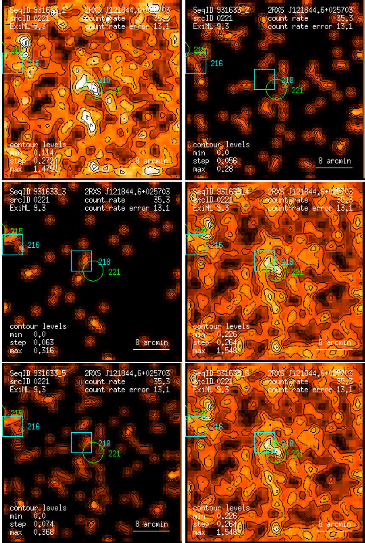
Figure 221: RASS 931633: detection 0221: band rate images, Gaussian filter: (1) PSPC channels 11 – 41, (2) 52 – 90, (3) 91 – 201, (4) 11 – 235, (5) 52 – 201, (6) 11 – 201. Broad band rates in counts/ks. Band rate contour levels in counts/ks/arcmin 2 .
