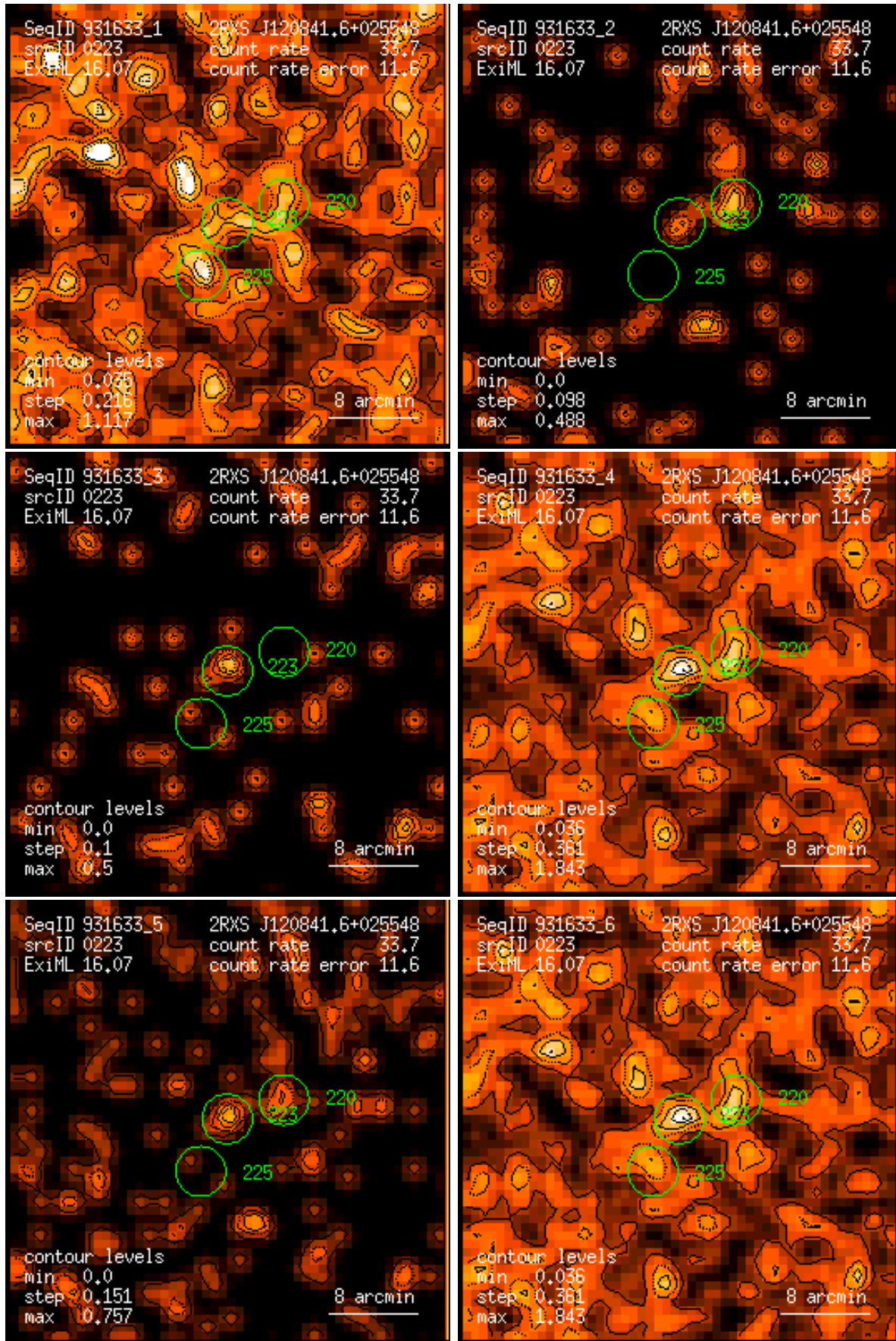
Figure 223: RASS 931633: detection 0223: band rate images, Gaussian filter: (1) PSPC channels 11 – 41, (2) 52 – 90, (3) 91 – 201, (4) 11 – 235, (5) 52 – 201, (6) 11 – 201. Broad band rates in counts/ks. Band rate contour levels in counts/ks/arcmin 2 .
