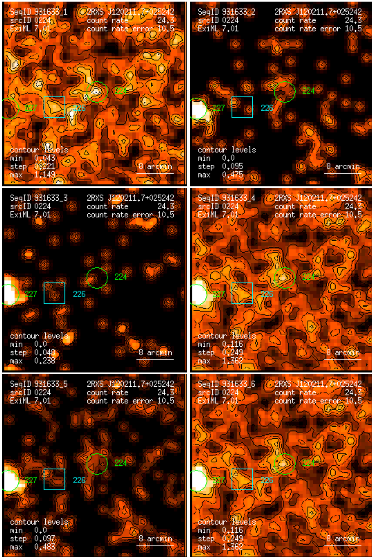
Figure 224: RASS 931633: detection 0224: band rate images, Gaussian filter: (1) PSPC channels 11 – 41, (2) 52 – 90, (3) 91 – 201, (4) 11 – 235, (5) 52 – 201, (6) 11 – 201. Broad band rates in counts/ks. Band rate contour levels in counts/ks/arcmin 2 .
