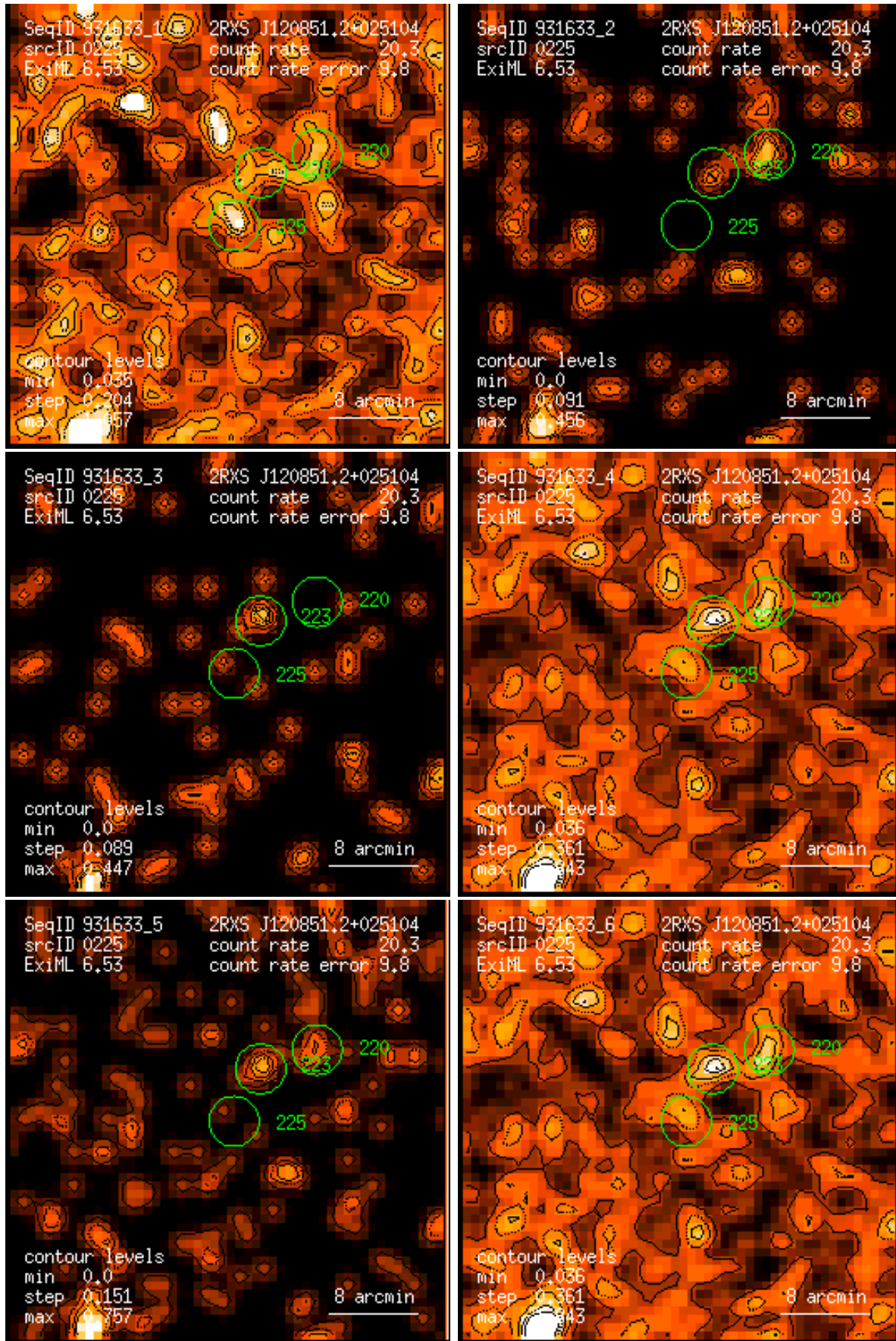
Figure 225: RASS 931633: detection 0225: band rate images, Gaussian filter: (1) PSPC channels 11 – 41, (2) 52 – 90, (3) 91 – 201, (4) 11 – 235, (5) 52 – 201, (6) 11 – 201. Broad band rates in counts/ks. Band rate contour levels in counts/ks/arcmin 2 .
