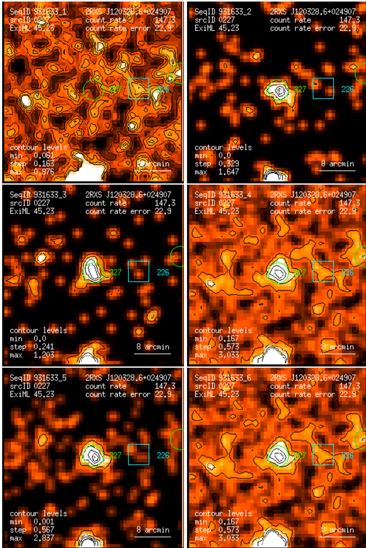
Figure 227: RASS 931633: detection 0227: band rate images, Gaussian filter: (1) PSPC channels 11 – 41, (2) 52 – 90, (3) 91 – 201, (4) 11 – 235, (5) 52 – 201, (6) 11 – 201. Broad band rates in counts/ks. Band rate contour levels in counts/ks/arcmin 2 .
