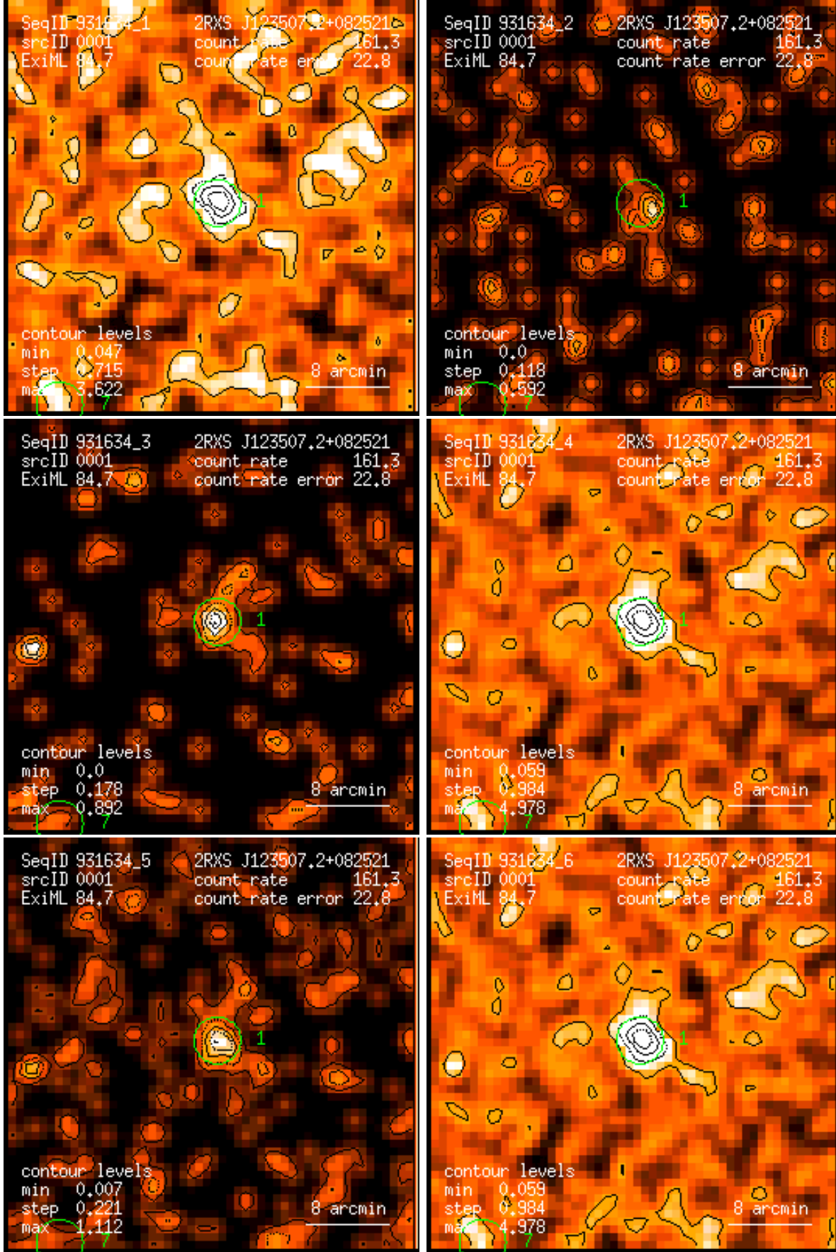
Figure 1: RASS 931634: detection 0001: band rate images, Gaussian filter: (1) PSPC channels 11 – 41, (2) 52 – 90, (3) 91 – 201, (4) 11 – 235, (5) 52 – 201, (6) 11 – 201. Broad band rates in counts/ks. Band rate contour levels in counts/ks/arcmin 2 .
