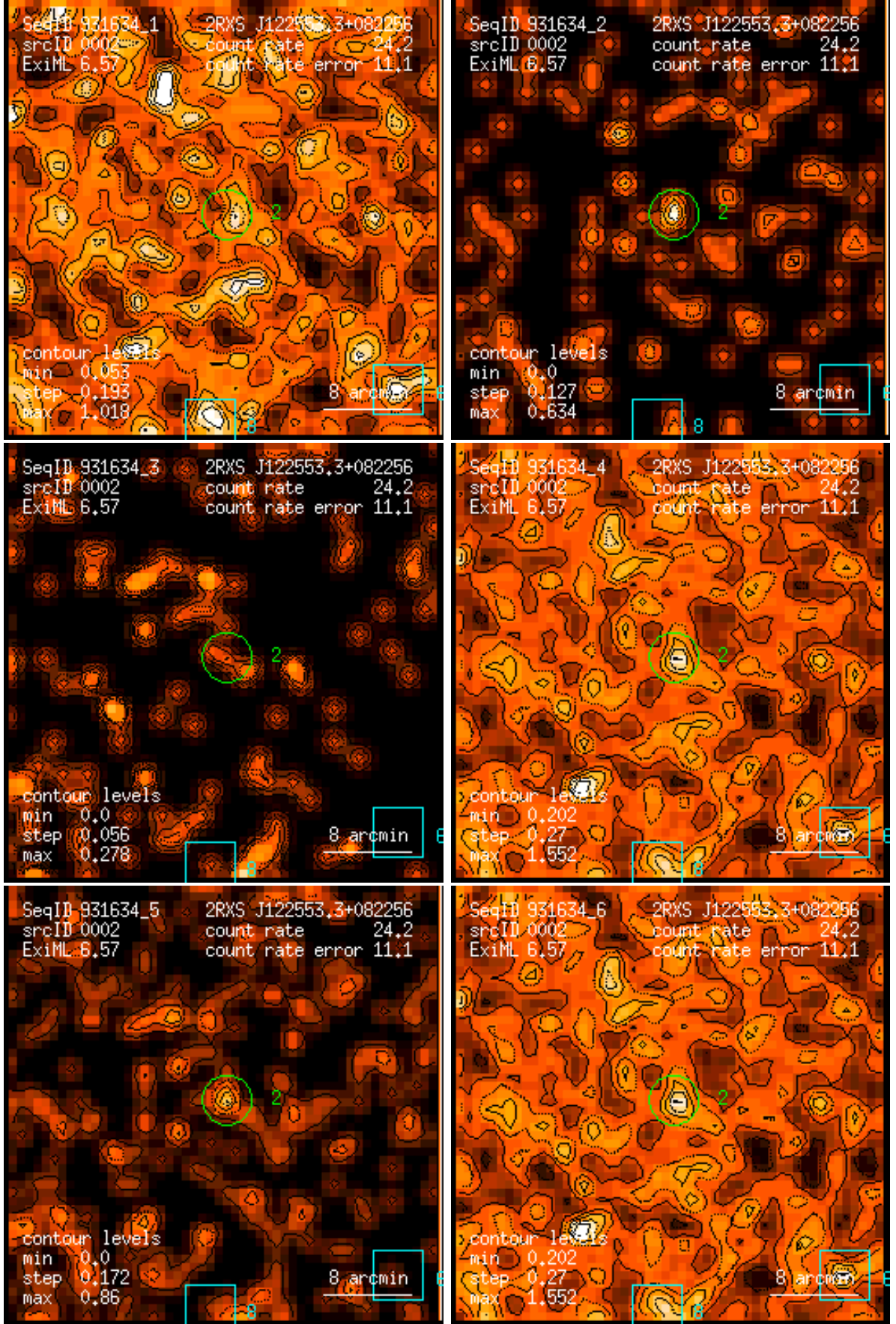
Figure 2: RASS 931634: detection 0002: band rate images, Gaussian filter: (1) PSPC channels 11 – 41, (2) 52 – 90, (3) 91 – 201, (4) 11 – 235, (5) 52 – 201, (6) 11 – 201. Broad band rates in counts/ks. Band rate contour levels in counts/ks/arcmin 2 .
