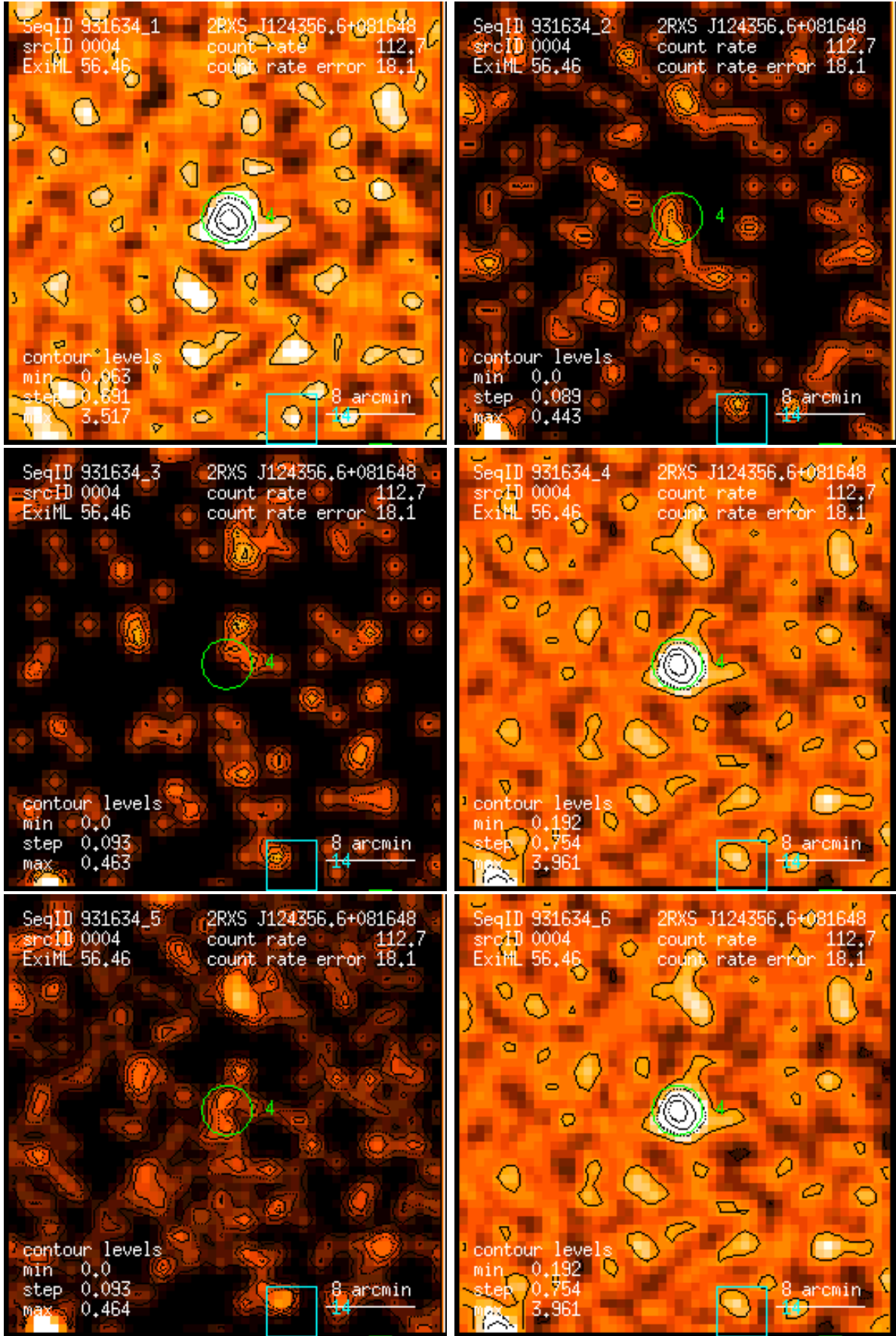
Figure 4: RASS 931634: detection 0004: band rate images, Gaussian filter: (1) PSPC channels 11 – 41, (2) 52 – 90, (3) 91 – 201, (4) 11 – 235, (5) 52 – 201, (6) 11 – 201. Broad band rates in counts/ks. Band rate contour levels in counts/ks/arcmin 2 .
