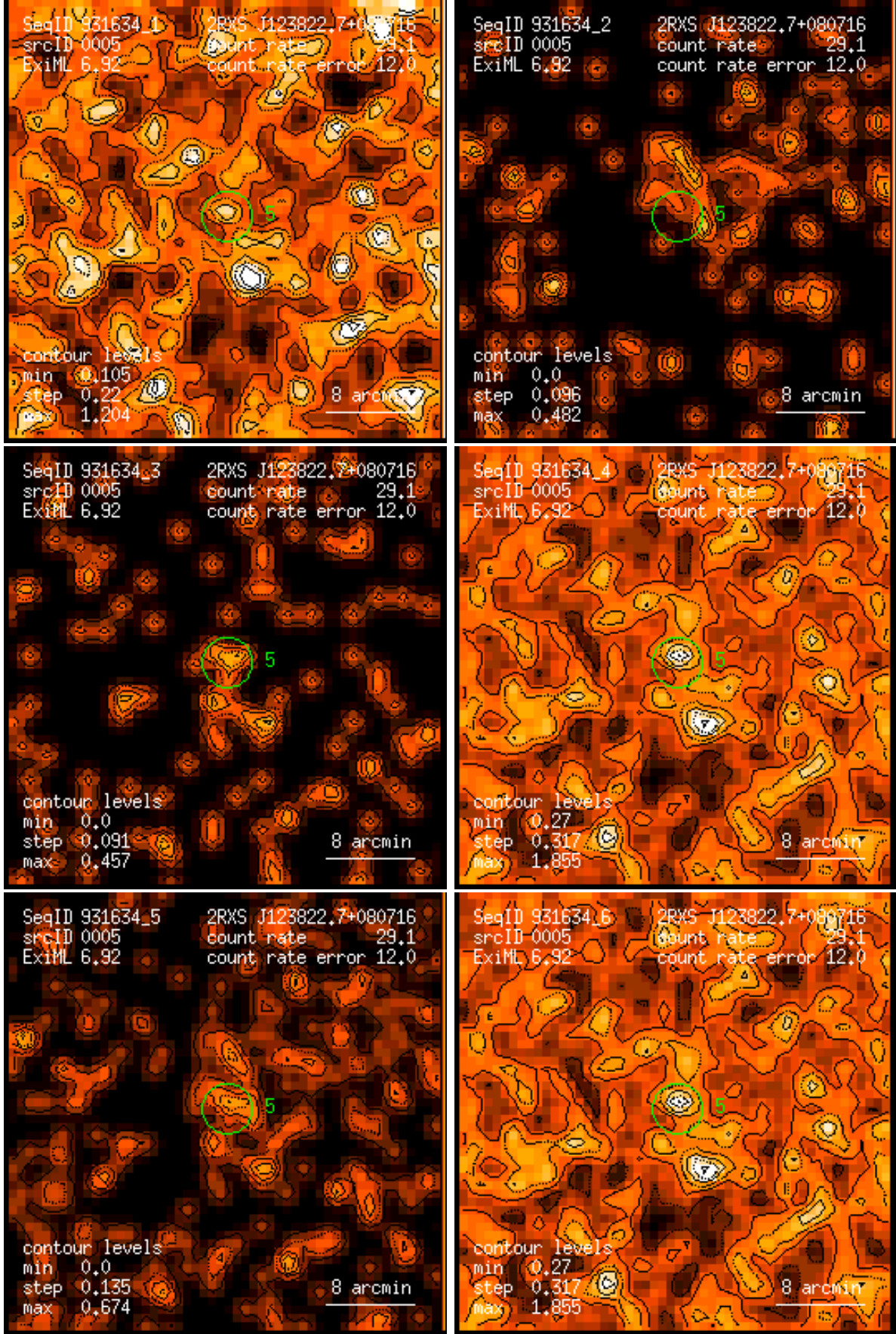
Figure 5: RASS 931634: detection 0005: band rate images, Gaussian filter: (1) PSPC channels 11 – 41, (2) 52 – 90, (3) 91 – 201, (4) 11 – 235, (5) 52 – 201, (6) 11 – 201. Broad band rates in counts/ks. Band rate contour levels in counts/ks/arcmin 2 .
