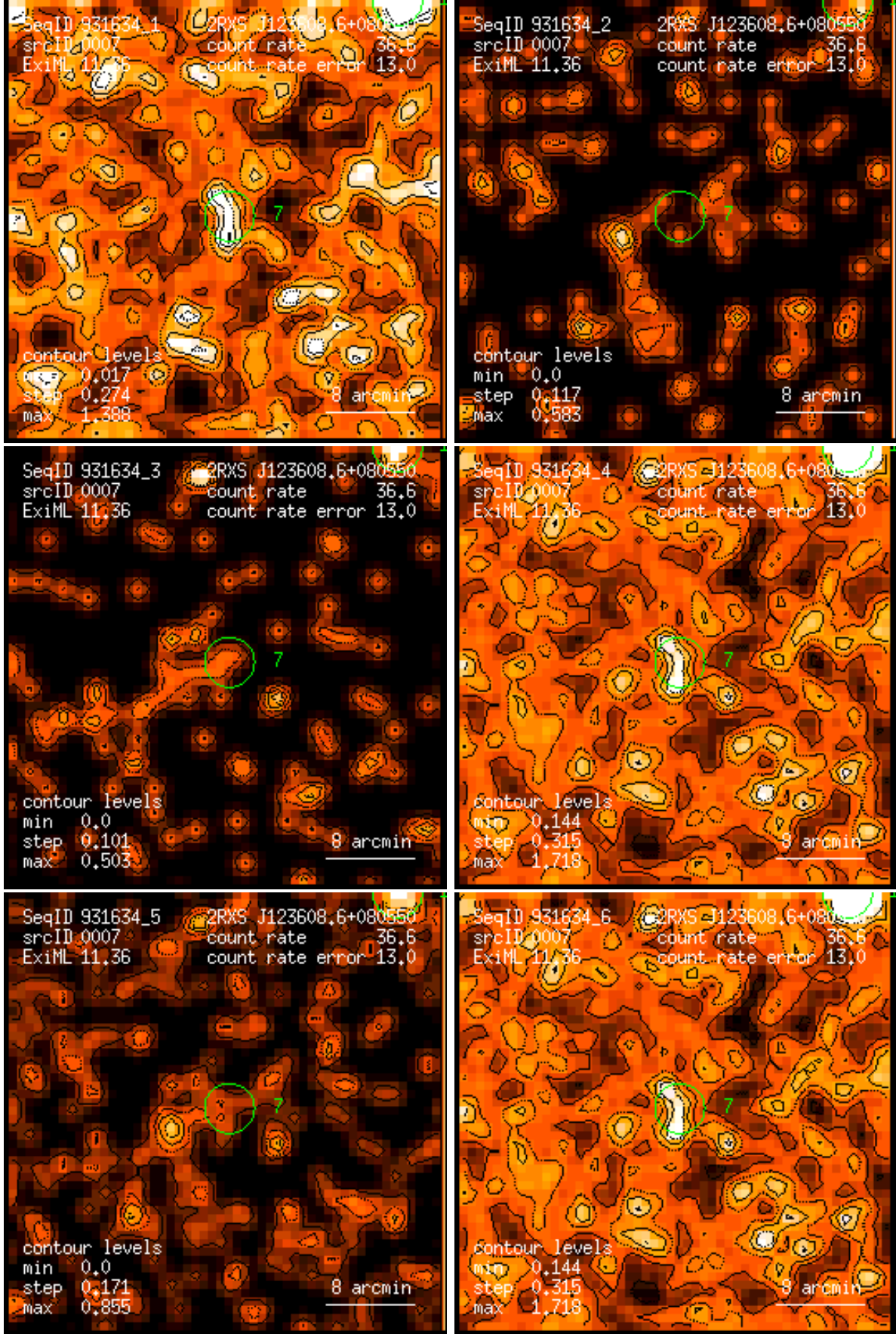
Figure 7: RASS 931634: detection 0007: band rate images, Gaussian filter: (1) PSPC channels 11 – 41, (2) 52 – 90, (3) 91 – 201, (4) 11 – 235, (5) 52 – 201, (6) 11 – 201. Broad band rates in counts/ks. Band rate contour levels in counts/ks/arcmin 2 .
