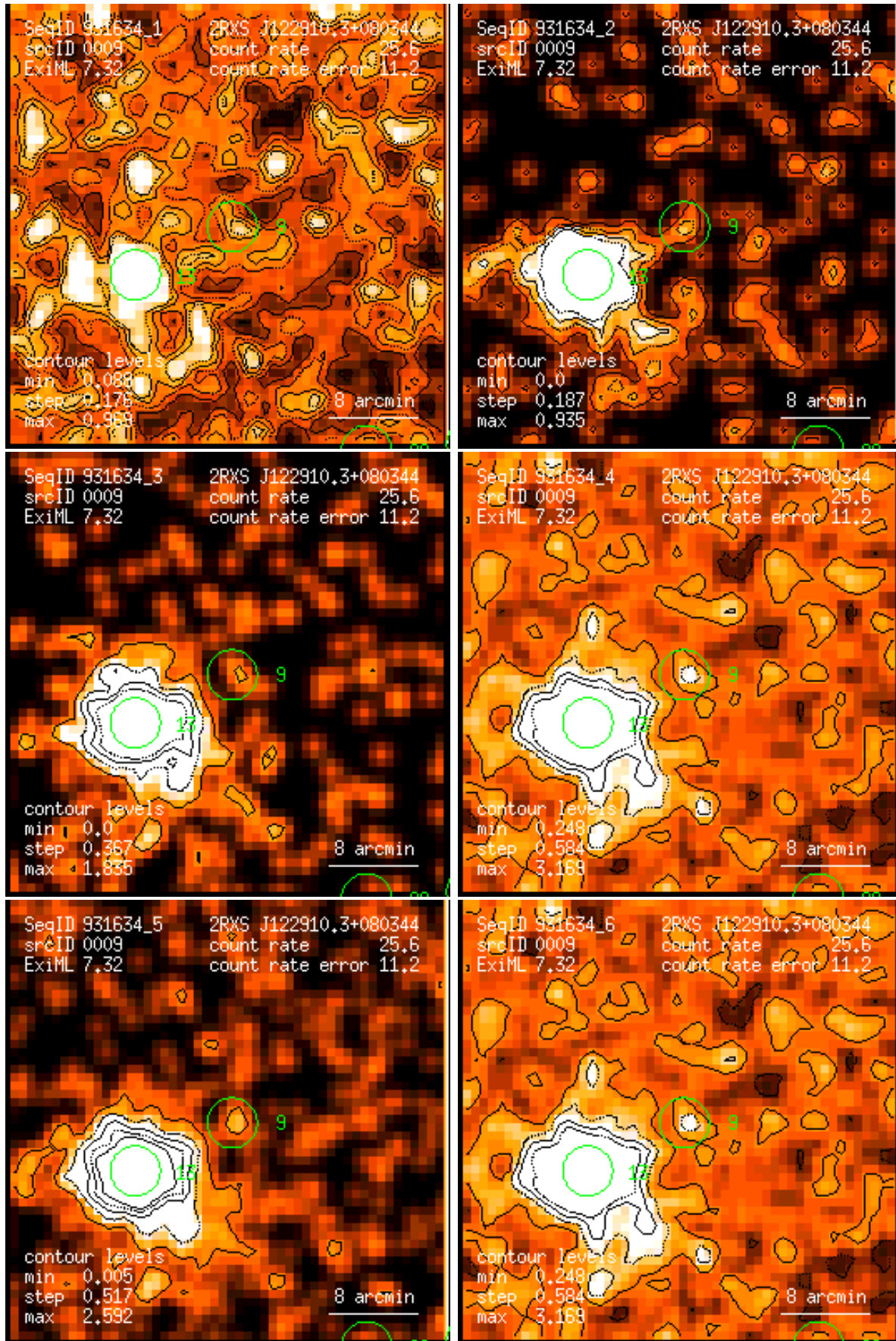
Figure 9: RASS 931634: detection 0009: band rate images, Gaussian filter: (1) PSPC channels 11 – 41, (2) 52 – 90, (3) 91 – 201, (4) 11 – 235, (5) 52 – 201, (6) 11 – 201. Broad band rates in counts/ks. Band rate contour levels in counts/ks/arcmin 2 .
