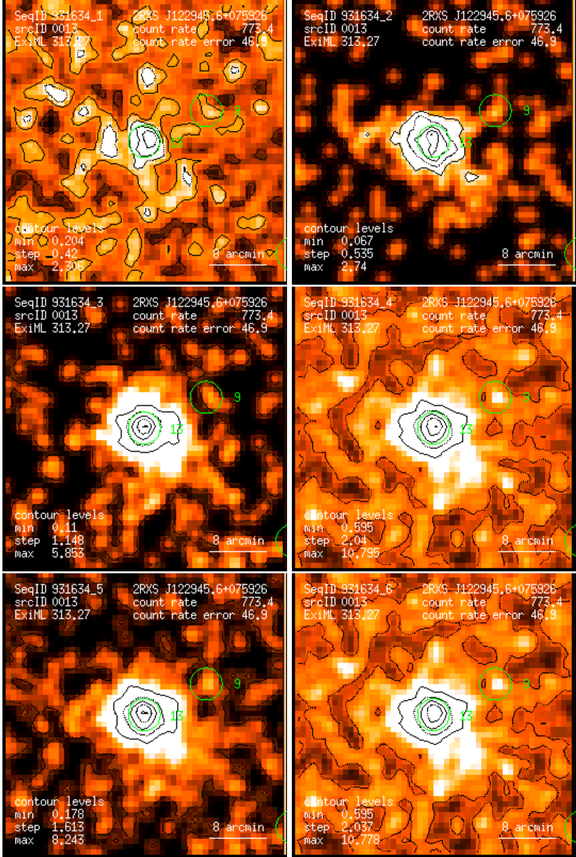
Figure 13: RASS 931634: detection 0013: band rate images, Gaussian filter: (1) PSPC channels 11 – 41, (2) 52 – 90, (3) 91 – 201, (4) 11 – 235, (5) 52 – 201, (6) 11 – 201. Broad band rates in counts/ks. Band rate contour levels in counts/ks/arcmin 2 .
