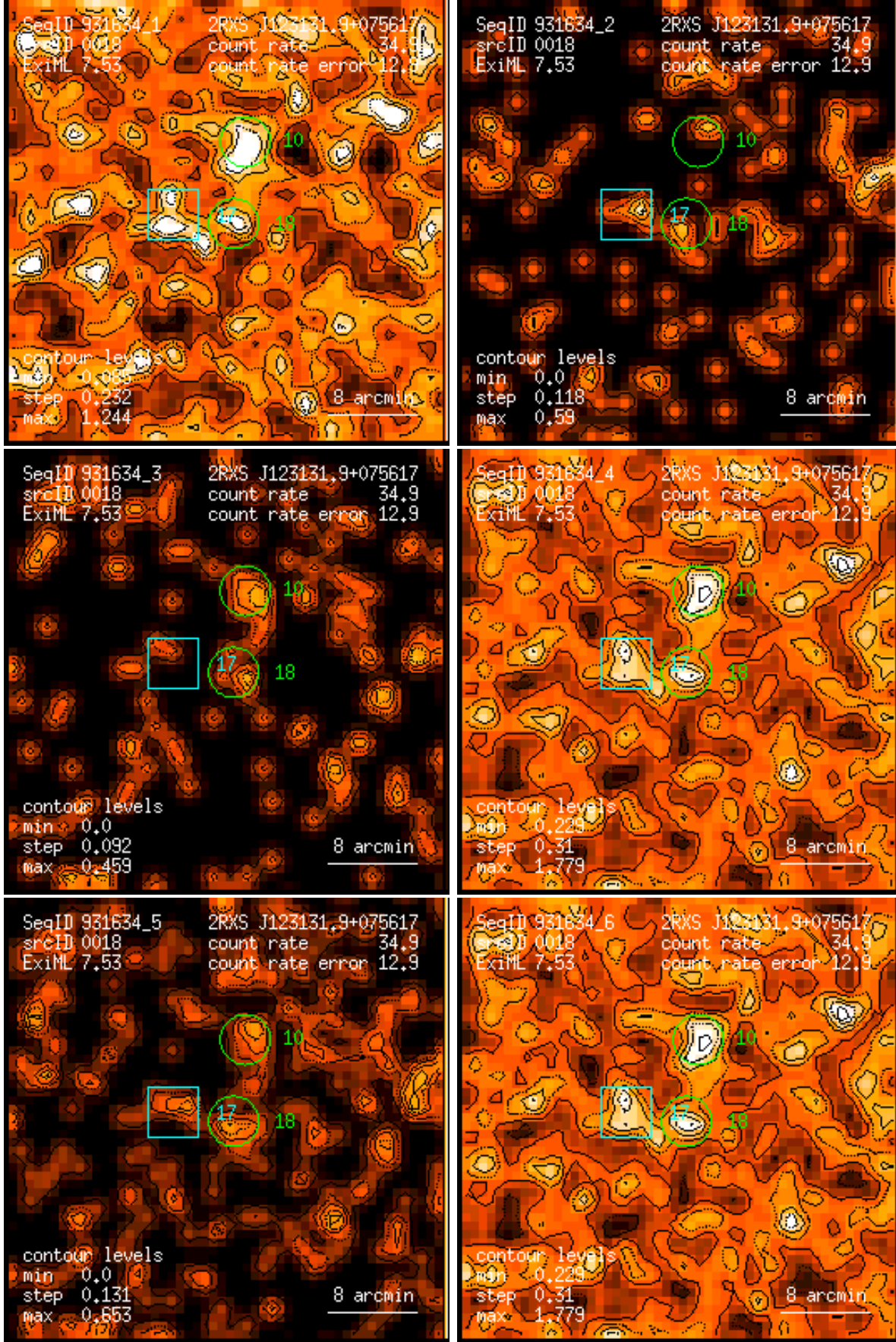
Figure 18: RASS 931634: detection 0018: band rate images, Gaussian filter: (1) PSPC channels 11 – 41, (2) 52 – 90, (3) 91 – 201, (4) 11 – 235, (5) 52 – 201, (6) 11 – 201. Broad band rates in counts/ks. Band rate contour levels in counts/ks/arcmin 2 .
