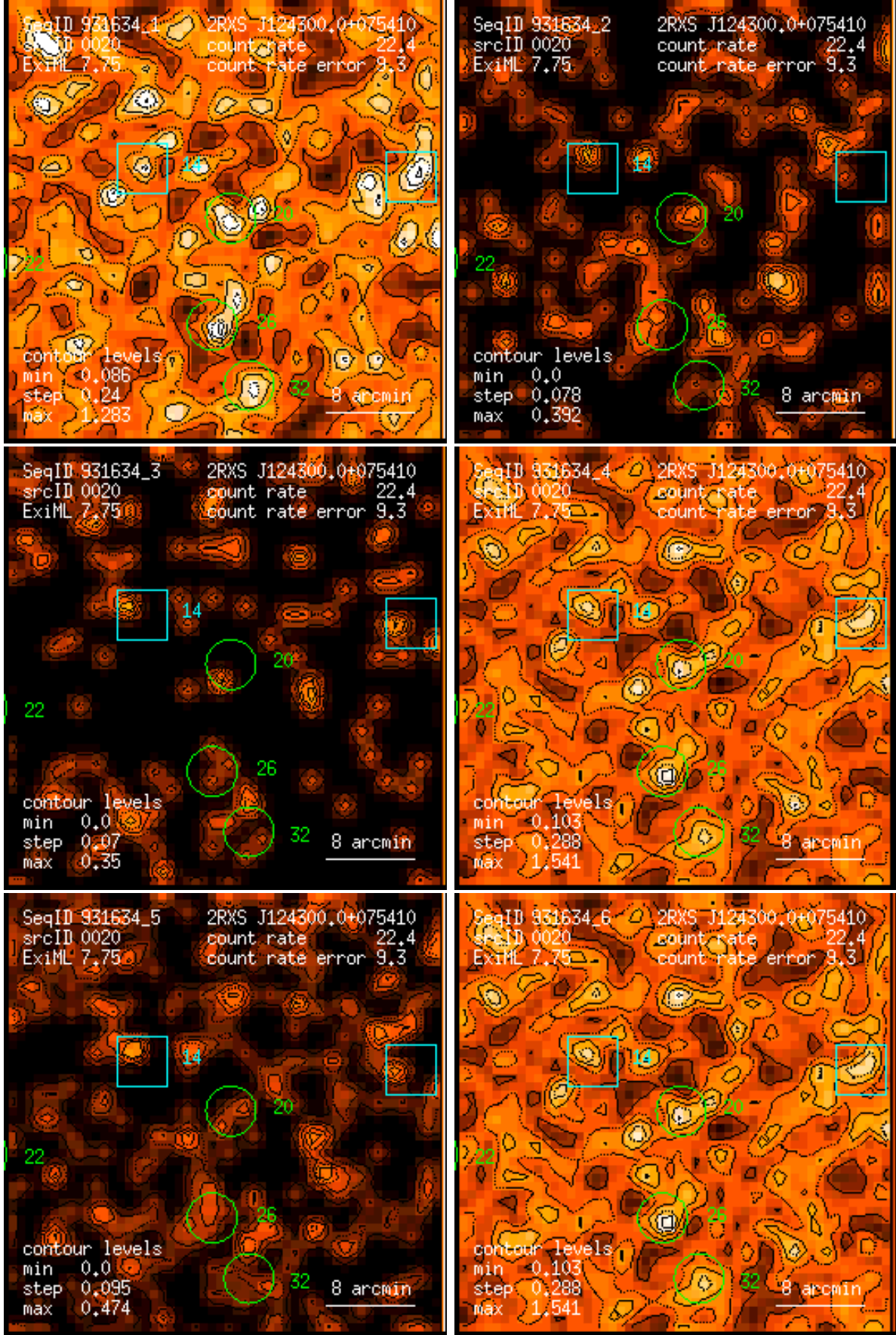
Figure 20: RASS 931634: detection 0020: band rate images, Gaussian filter: (1) PSPC channels 11 – 41, (2) 52 – 90, (3) 91 – 201, (4) 11 – 235, (5) 52 – 201, (6) 11 – 201. Broad band rates in counts/ks. Band rate contour levels in counts/ks/arcmin 2 .
