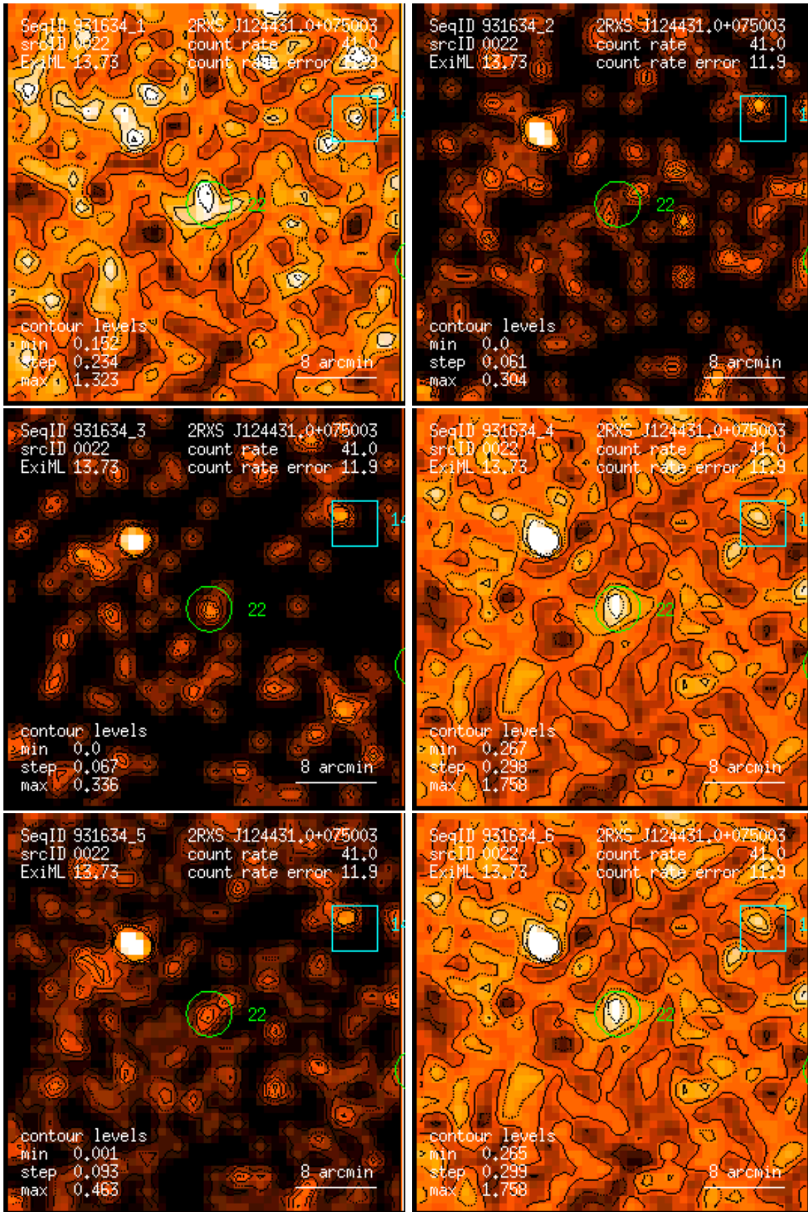
Figure 22: RASS 931634: detection 0022: band rate images, Gaussian filter: (1) PSPC channels 11 – 41, (2) 52 – 90, (3) 91 – 201, (4) 11 – 235, (5) 52 – 201, (6) 11 – 201. Broad band rates in counts/ks. Band rate contour levels in counts/ks/arcmin 2 .
