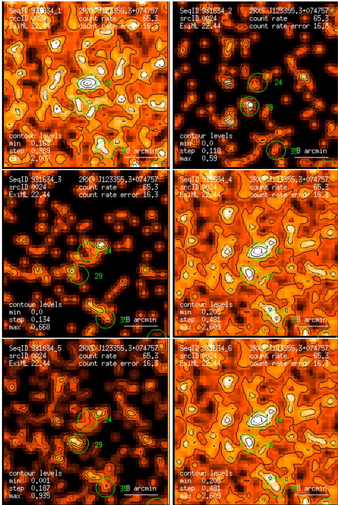
Figure 24: RASS 931634: detection 0024: band rate images, Gaussian filter: (1) PSPC channels 11 – 41, (2) 52 – 90, (3) 91 – 201, (4) 11 – 235, (5) 52 – 201, (6) 11 – 201. Broad band rates in counts/ks. Band rate contour levels in counts/ks/arcmin 2 .
