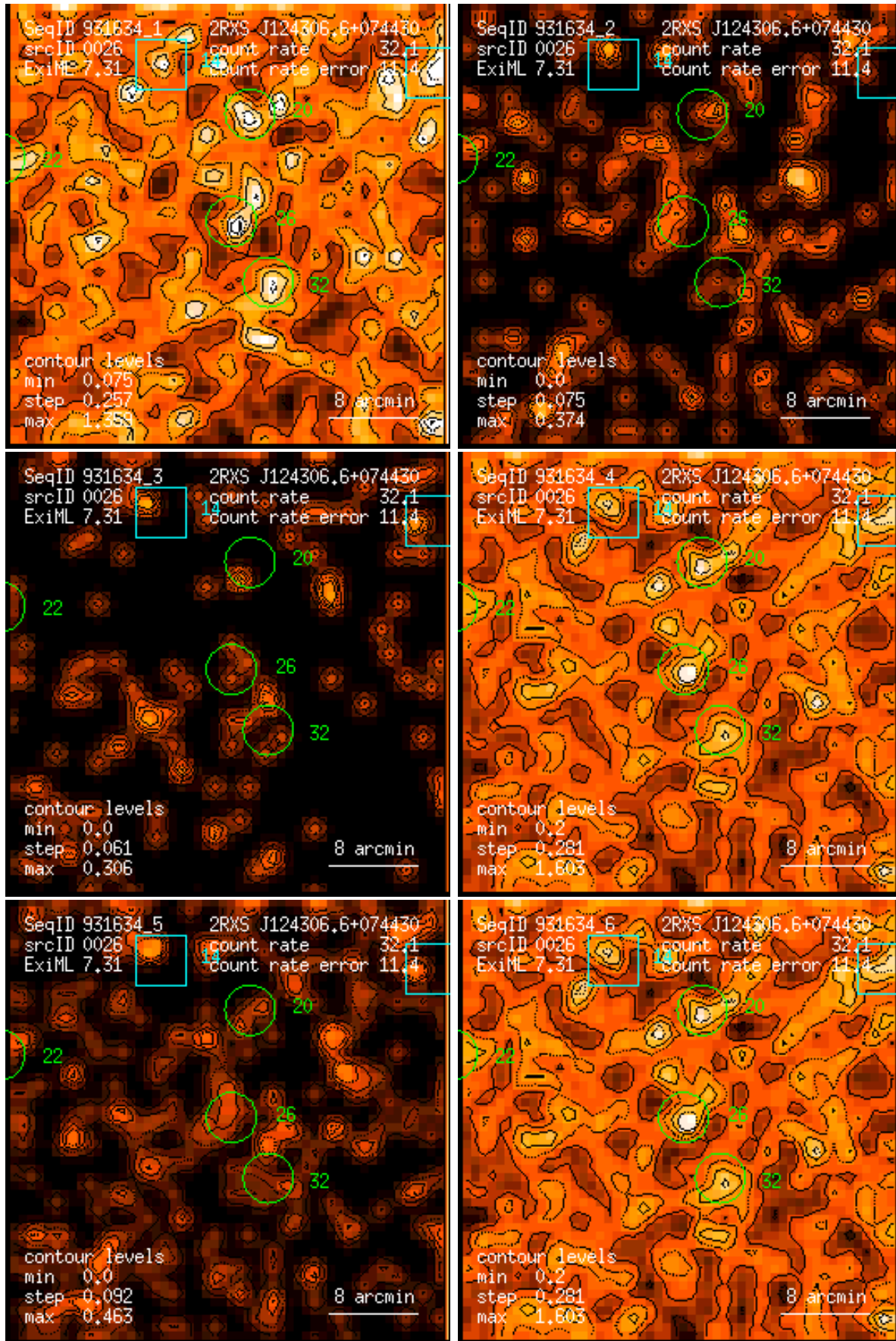
Figure 26: RASS 931634: detection 0026: band rate images, Gaussian filter: (1) PSPC channels 11 – 41, (2) 52 – 90, (3) 91 – 201, (4) 11 – 235, (5) 52 – 201, (6) 11 – 201. Broad band rates in counts/ks. Band rate contour levels in counts/ks/arcmin 2 .
