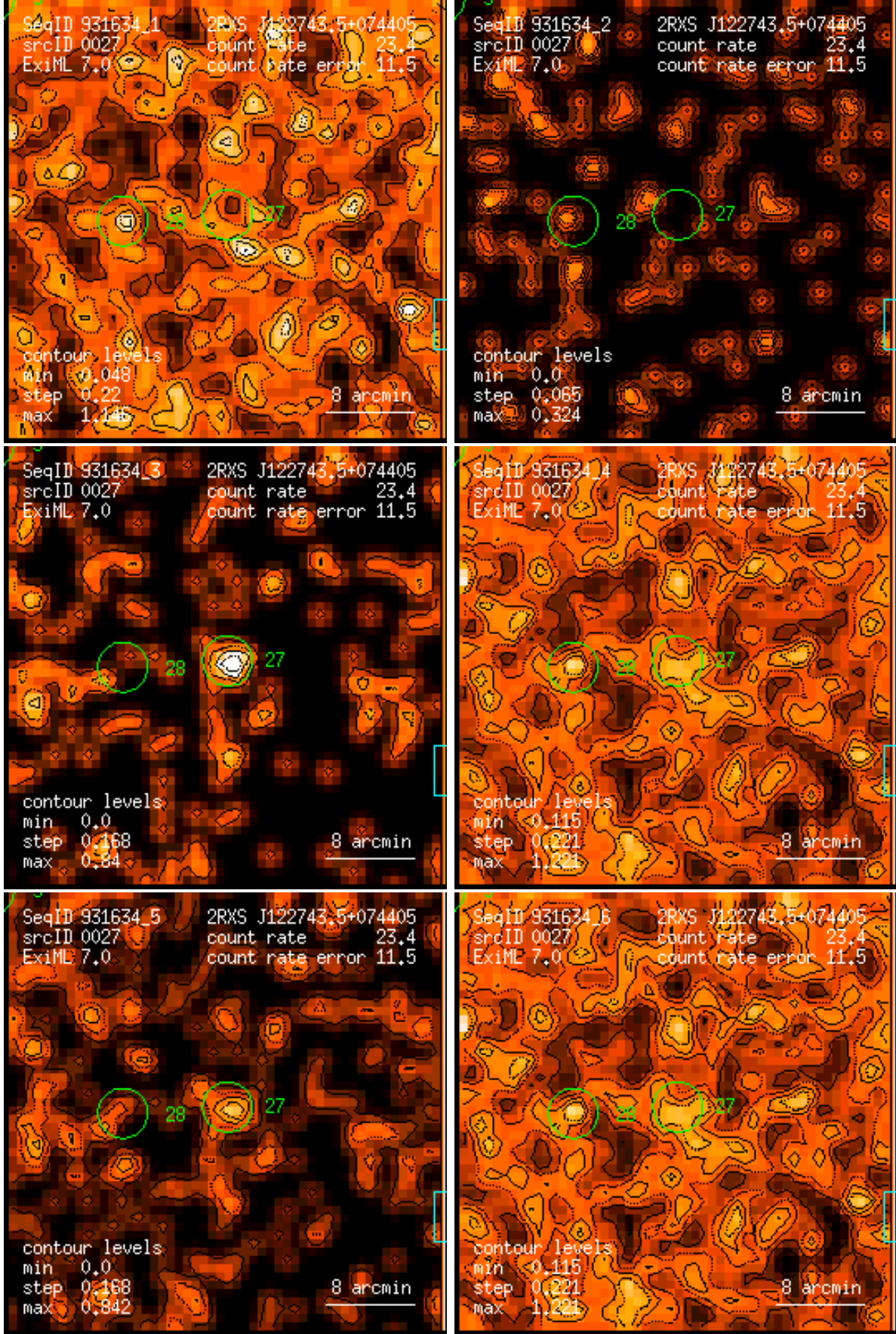
Figure 27: RASS 931634: detection 0027: band rate images, Gaussian filter: (1) PSPC channels 11 – 41, (2) 52 – 90, (3) 91 – 201, (4) 11 – 235, (5) 52 – 201, (6) 11 – 201. Broad band rates in counts/ks. Band rate contour levels in counts/ks/arcmin 2 .
