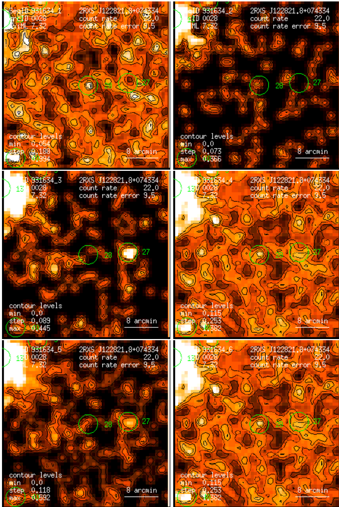
Figure 28: RASS 931634: detection 0028: band rate images, Gaussian filter: (1) PSPC channels 11 – 41, (2) 52 – 90, (3) 91 – 201, (4) 11 – 235, (5) 52 – 201, (6) 11 – 201. Broad band rates in counts/ks. Band rate contour levels in counts/ks/arcmin 2 .
