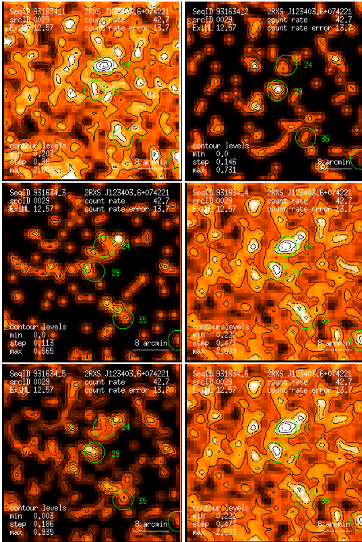
Figure 29: RASS 931634: detection 0029: band rate images, Gaussian filter: (1) PSPC channels 11 – 41, (2) 52 – 90, (3) 91 – 201, (4) 11 – 235, (5) 52 – 201, (6) 11 – 201. Broad band rates in counts/ks. Band rate contour levels in counts/ks/arcmin 2 .
