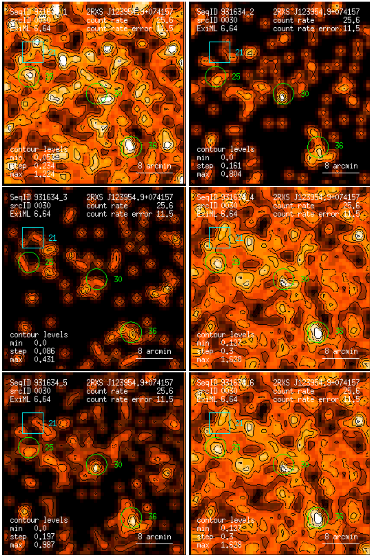
Figure 30: RASS 931634: detection 0030: band rate images, Gaussian filter: (1) PSPC channels 11 – 41, (2) 52 – 90, (3) 91 – 201, (4) 11 – 235, (5) 52 – 201, (6) 11 – 201. Broad band rates in counts/ks. Band rate contour levels in counts/ks/arcmin 2 .
