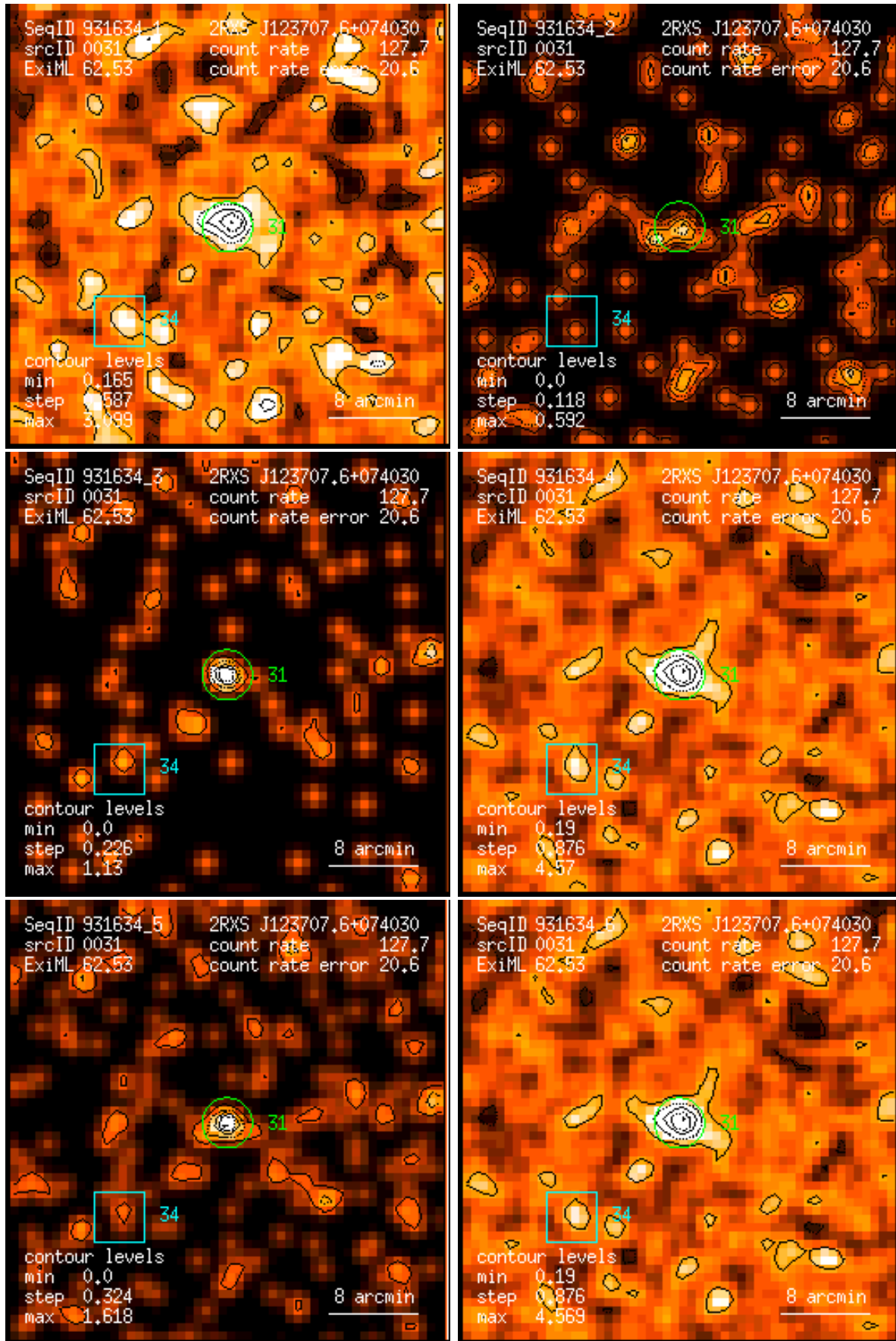
Figure 31: RASS 931634: detection 0031: band rate images, Gaussian filter: (1) PSPC channels 11 – 41, (2) 52 – 90, (3) 91 – 201, (4) 11 – 235, (5) 52 – 201, (6) 11 – 201. Broad band rates in counts/ks. Band rate contour levels in counts/ks/arcmin 2 .
