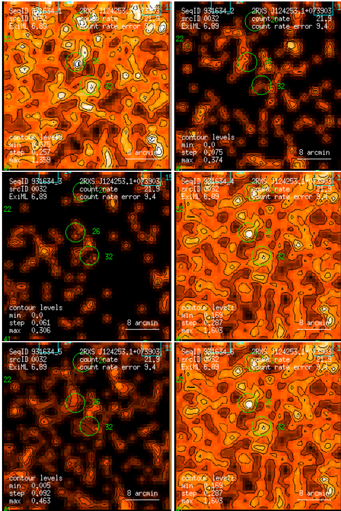
Figure 32: RASS 931634: detection 0032: band rate images, Gaussian filter: (1) PSPC channels 11 – 41, (2) 52 – 90, (3) 91 – 201, (4) 11 – 235, (5) 52 – 201, (6) 11 – 201. Broad band rates in counts/ks. Band rate contour levels in counts/ks/arcmin 2 .
