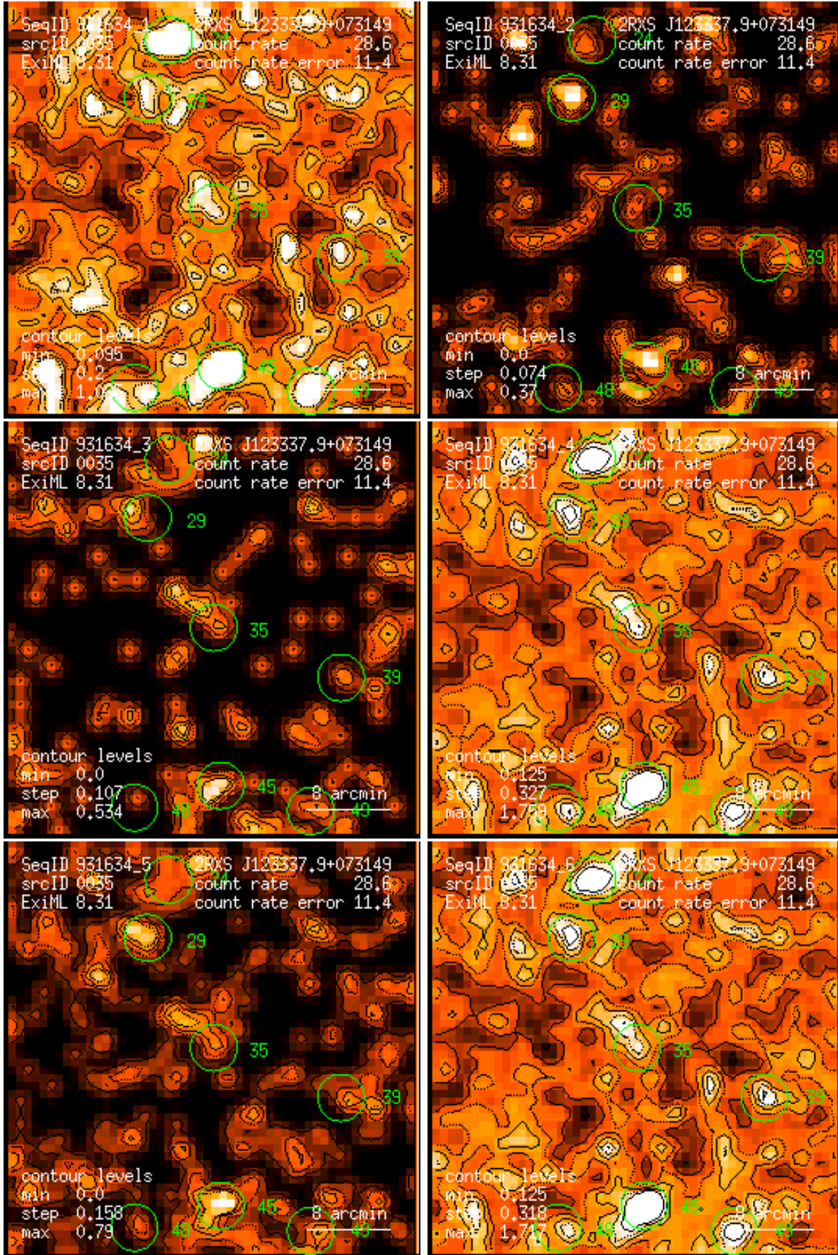
Figure 35: RASS 931634: detection 0035: band rate images, Gaussian filter: (1) PSPC channels 11 – 41, (2) 52 – 90, (3) 91 – 201, (4) 11 – 235, (5) 52 – 201, (6) 11 – 201. Broad band rates in counts/ks. Band rate contour levels in counts/ks/arcmin 2 .
