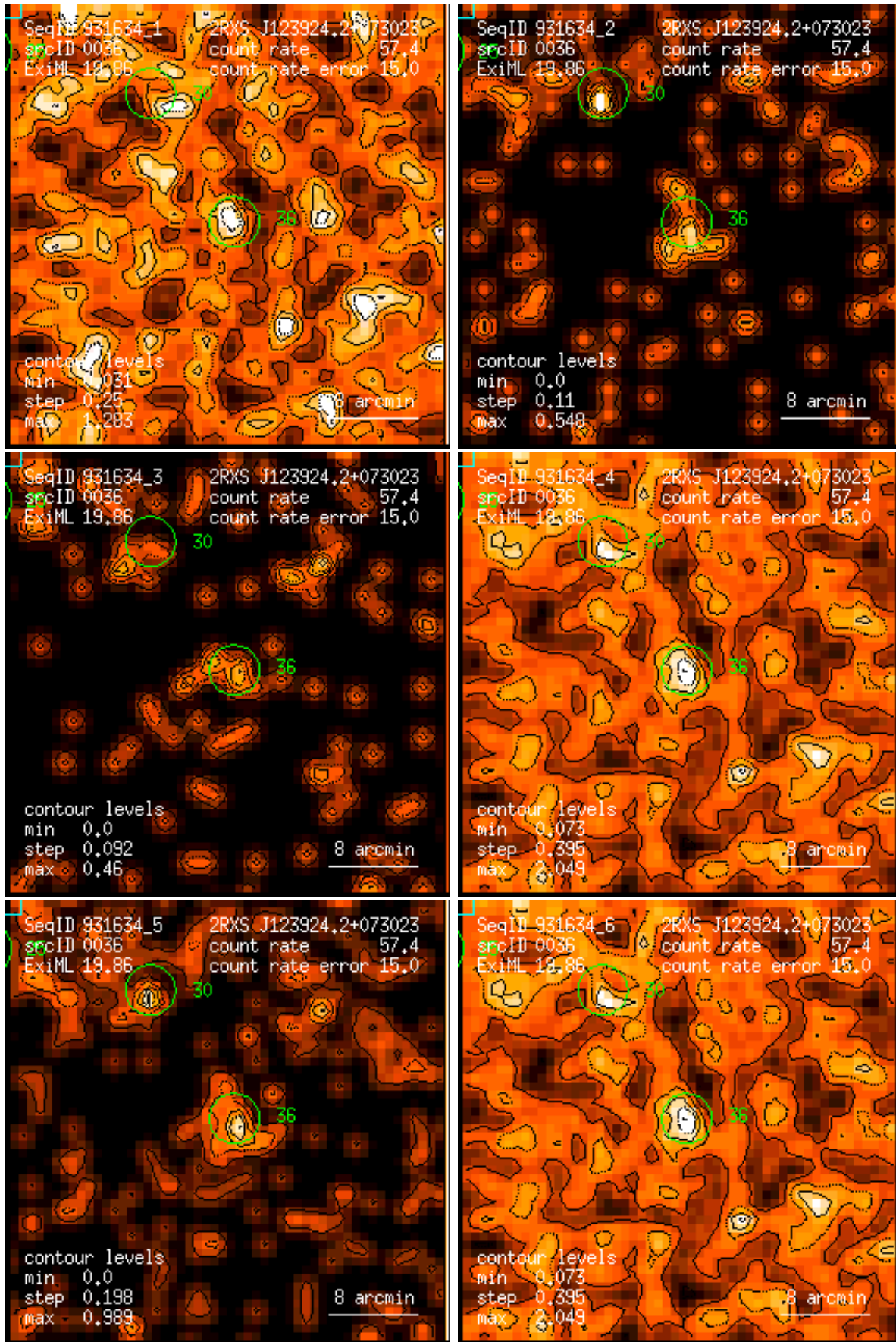
Figure 36: RASS 931634: detection 0036: band rate images, Gaussian filter: (1) PSPC channels 11 – 41, (2) 52 – 90, (3) 91 – 201, (4) 11 – 235, (5) 52 – 201, (6) 11 – 201. Broad band rates in counts/ks. Band rate contour levels in counts/ks/arcmin 2 .
