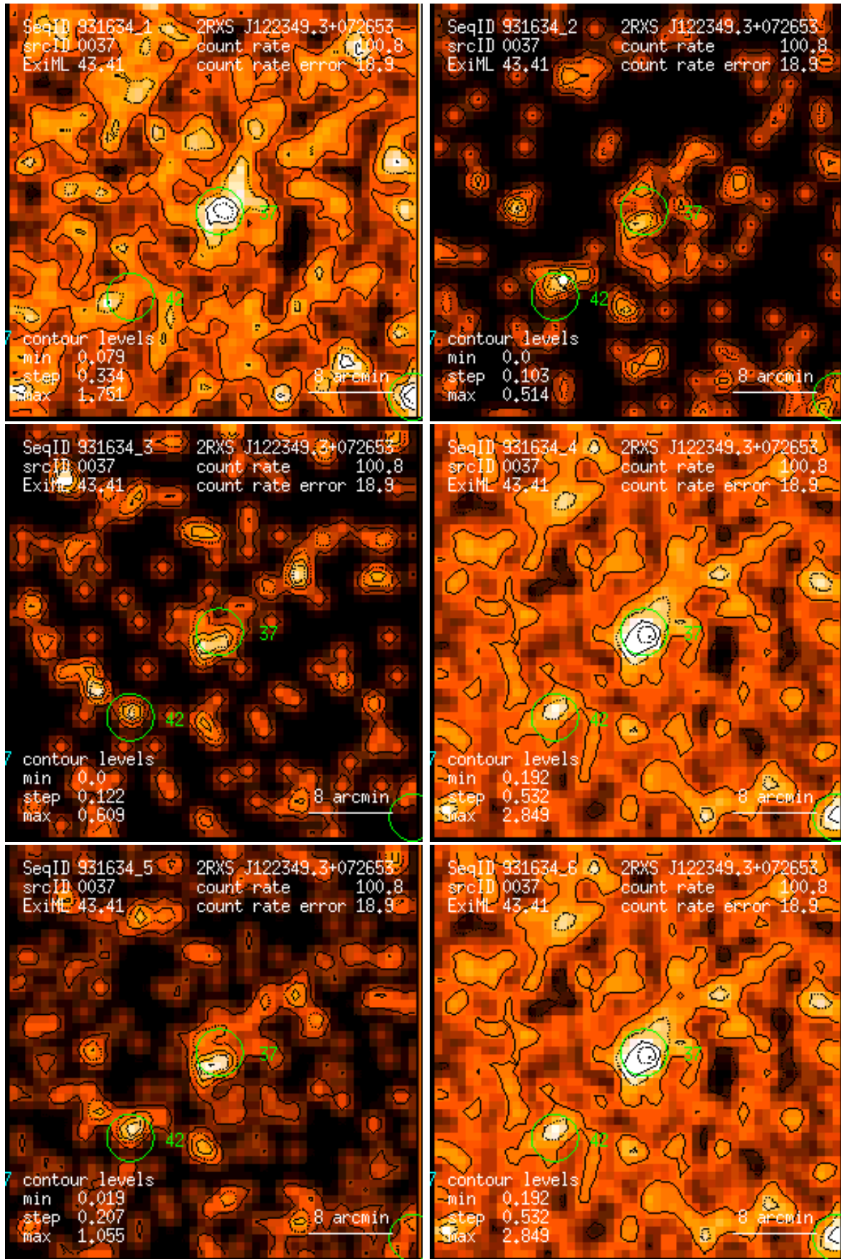
Figure 37: RASS 931634: detection 0037: band rate images, Gaussian filter: (1) PSPC channels 11 – 41, (2) 52 – 90, (3) 91 – 201, (4) 11 – 235, (5) 52 – 201, (6) 11 – 201. Broad band rates in counts/ks. Band rate contour levels in counts/ks/arcmin 2 .
