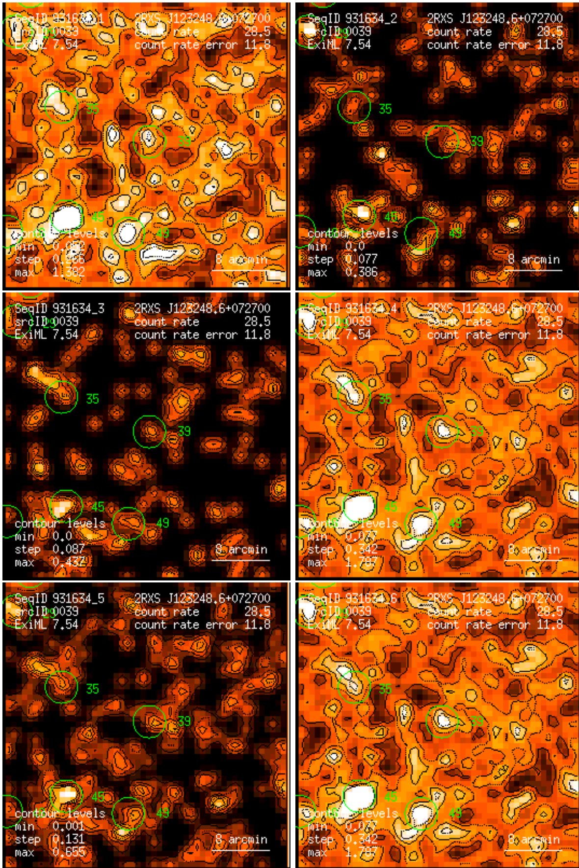
Figure 39: RASS 931634: detection 0039: band rate images, Gaussian filter: (1) PSPC channels 11 – 41, (2) 52 – 90, (3) 91 – 201, (4) 11 – 235, (5) 52 – 201, (6) 11 – 201. Broad band rates in counts/ks. Band rate contour levels in counts/ks/arcmin 2 .
