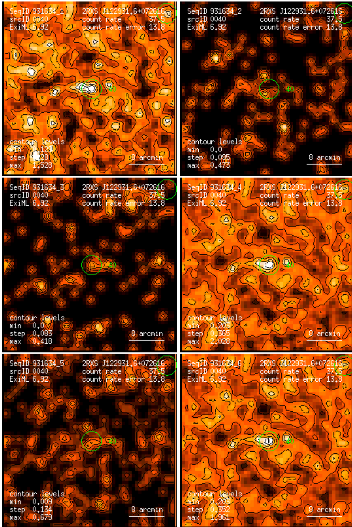
Figure 40: RASS 931634: detection 0040: band rate images, Gaussian filter: (1) PSPC channels 11 – 41, (2) 52 – 90, (3) 91 – 201, (4) 11 – 235, (5) 52 – 201, (6) 11 – 201. Broad band rates in counts/ks. Band rate contour levels in counts/ks/arcmin 2 .
