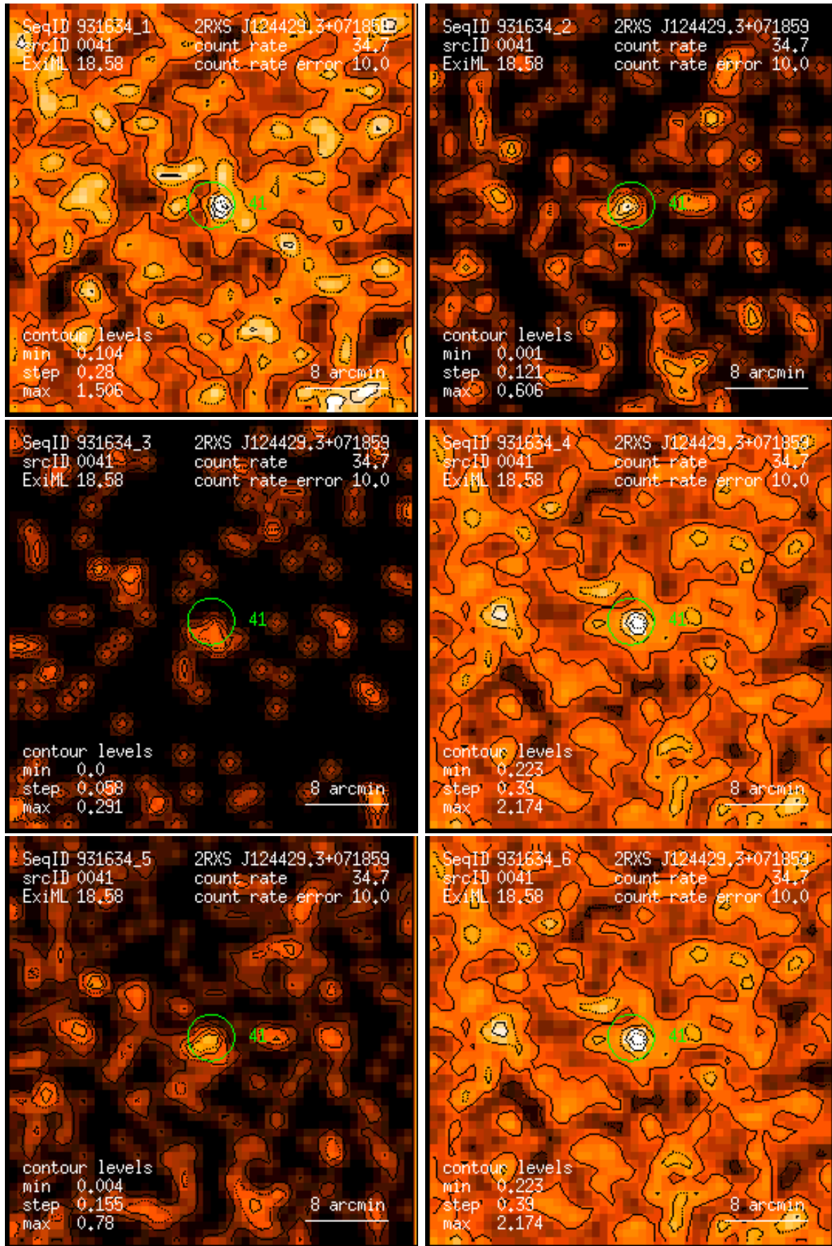
Figure 41: RASS 931634: detection 0041: band rate images, Gaussian filter: (1) PSPC channels 11 – 41, (2) 52 – 90, (3) 91 – 201, (4) 11 – 235, (5) 52 – 201, (6) 11 – 201. Broad band rates in counts/ks. Band rate contour levels in counts/ks/arcmin 2 .
