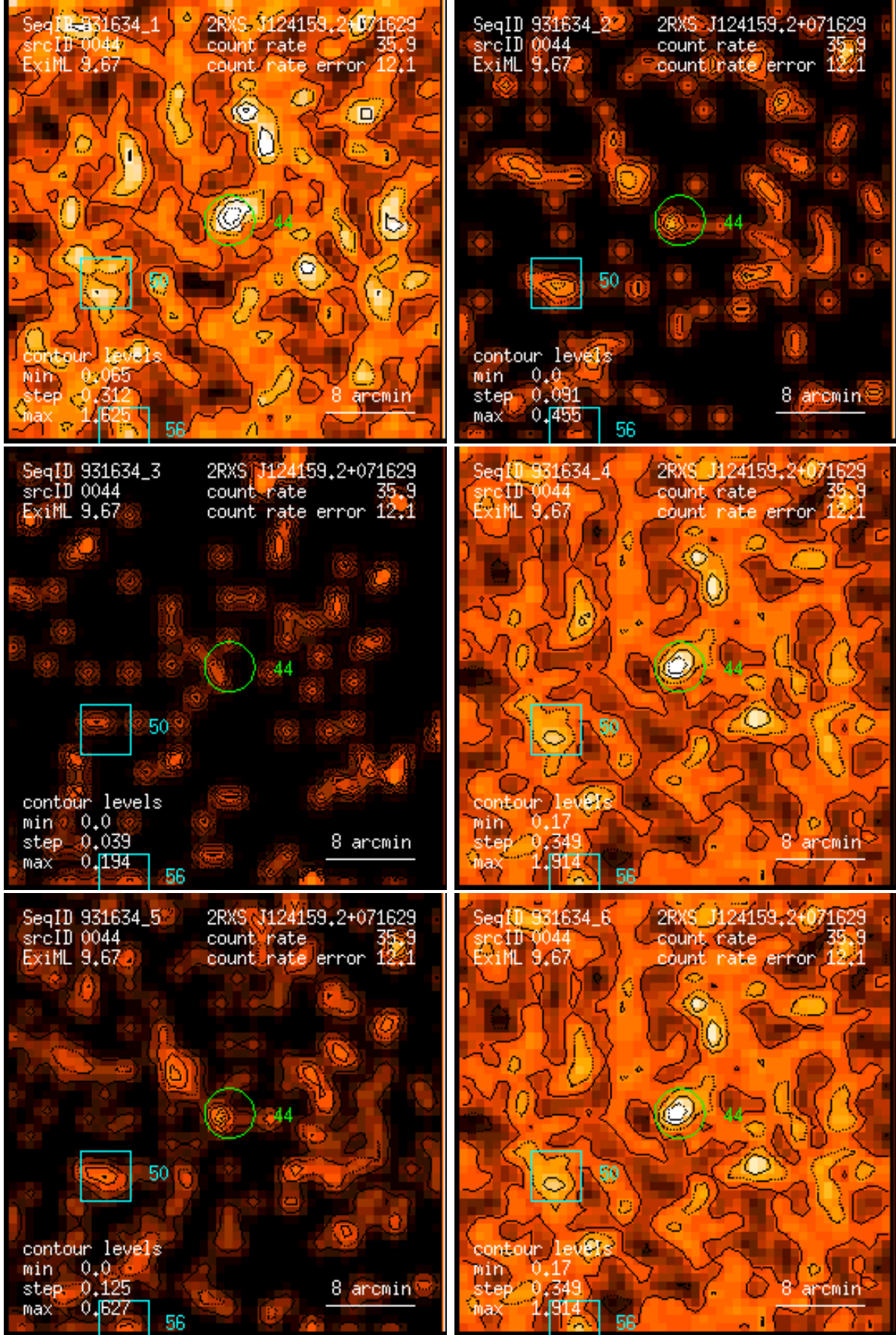
Figure 44: RASS 931634: detection 0044: band rate images, Gaussian filter: (1) PSPC channels 11 – 41, (2) 52 – 90, (3) 91 – 201, (4) 11 – 235, (5) 52 – 201, (6) 11 – 201. Broad band rates in counts/ks. Band rate contour levels in counts/ks/arcmin 2 .
