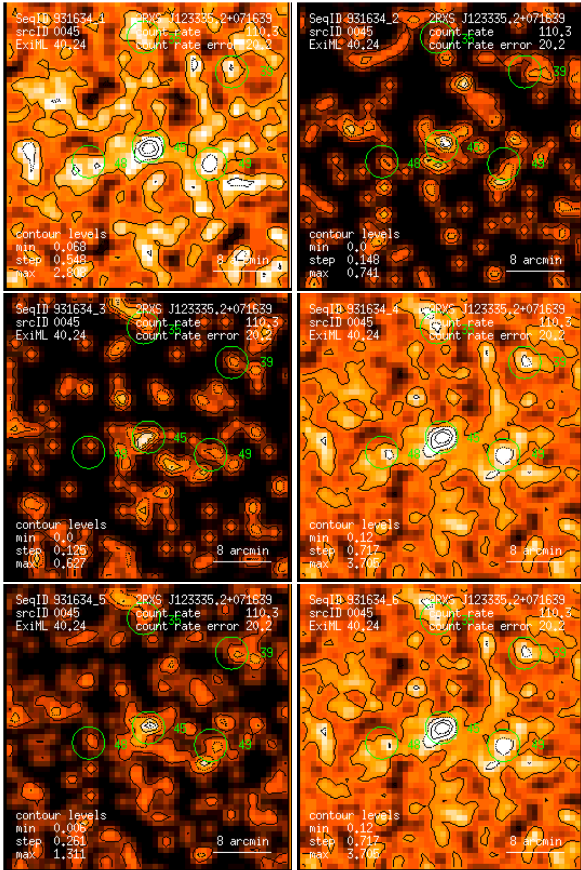
Figure 45: RASS 931634: detection 0045: band rate images, Gaussian filter: (1) PSPC channels 11 – 41, (2) 52 – 90, (3) 91 – 201, (4) 11 – 235, (5) 52 – 201, (6) 11 – 201. Broad band rates in counts/ks. Band rate contour levels in counts/ks/arcmin 2 .
