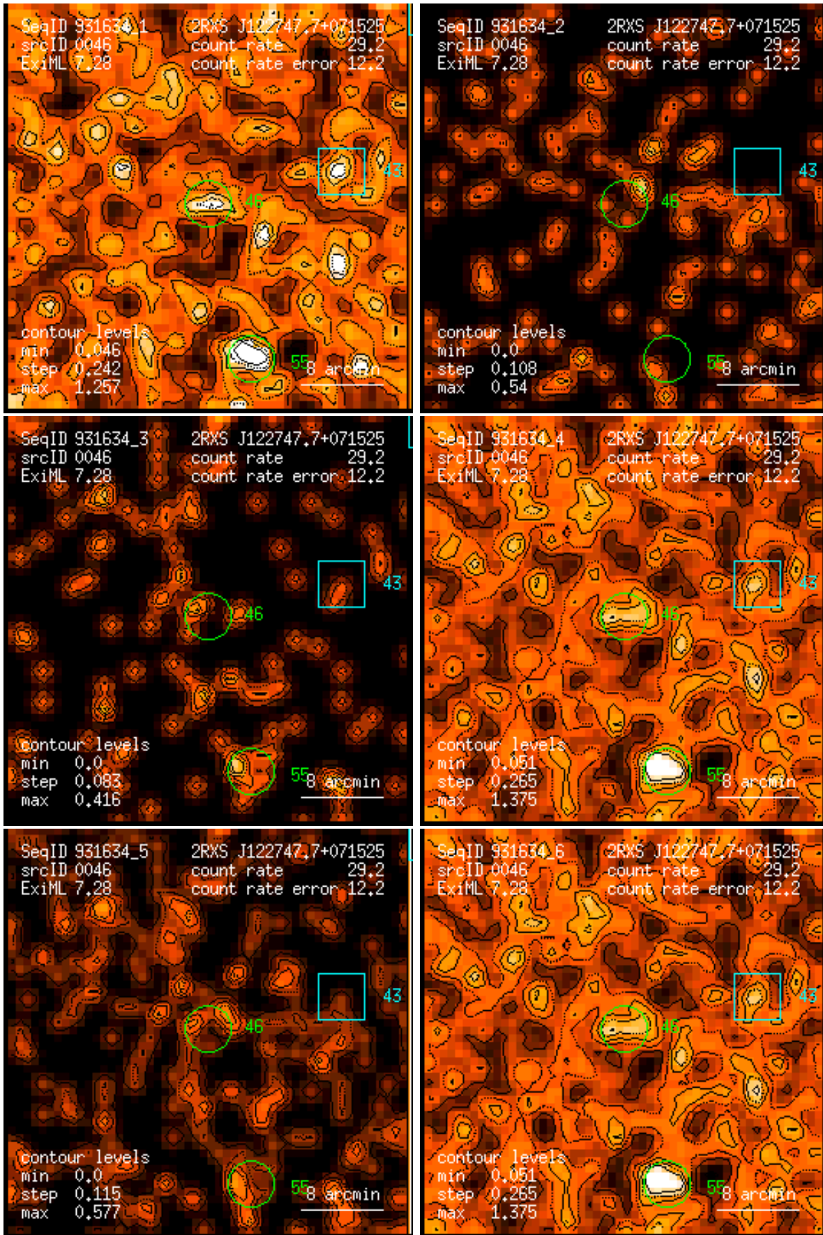
Figure 46: RASS 931634: detection 0046: band rate images, Gaussian filter: (1) PSPC channels 11 – 41, (2) 52 – 90, (3) 91 – 201, (4) 11 – 235, (5) 52 – 201, (6) 11 – 201. Broad band rates in counts/ks. Band rate contour levels in counts/ks/arcmin 2 .
