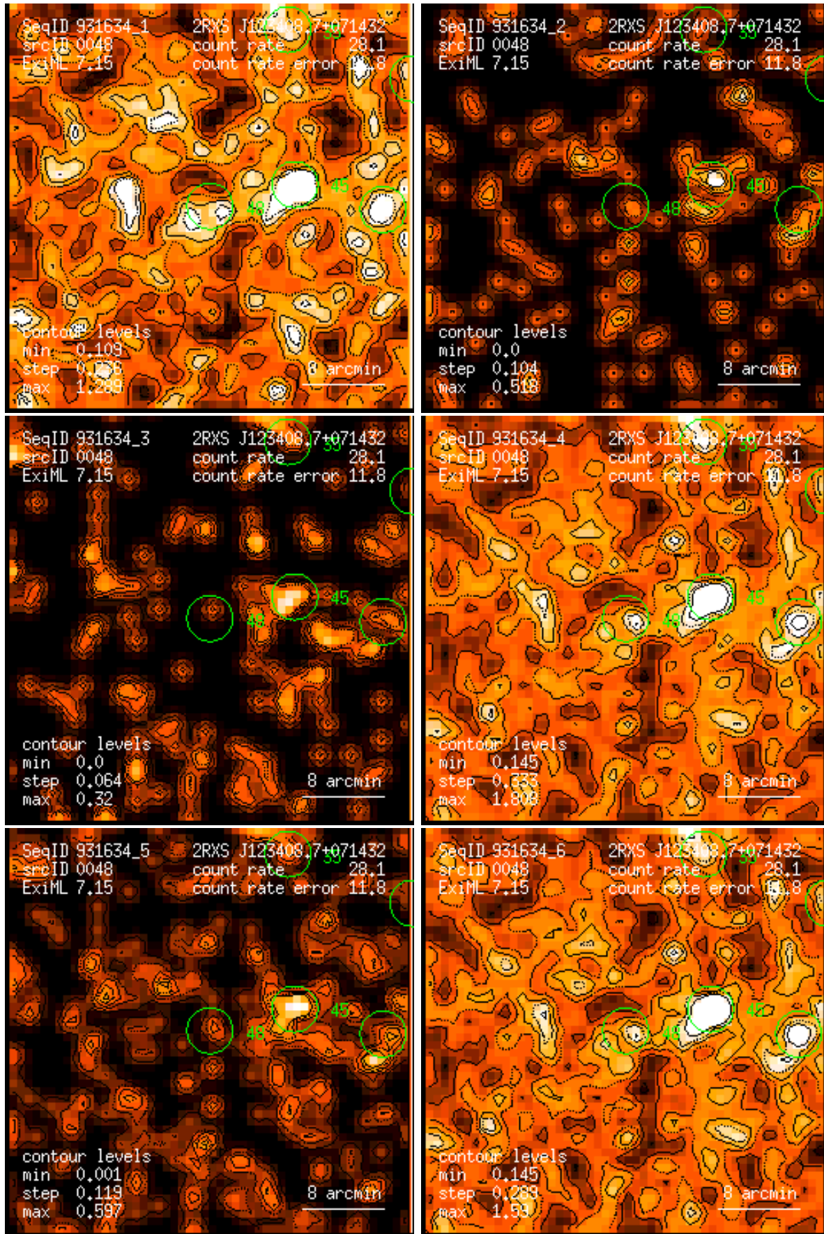
Figure 48: RASS 931634: detection 0048: band rate images, Gaussian filter: (1) PSPC channels 11 – 41, (2) 52 – 90, (3) 91 – 201, (4) 11 – 235, (5) 52 – 201, (6) 11 – 201. Broad band rates in counts/ks. Band rate contour levels in counts/ks/arcmin 2 .
