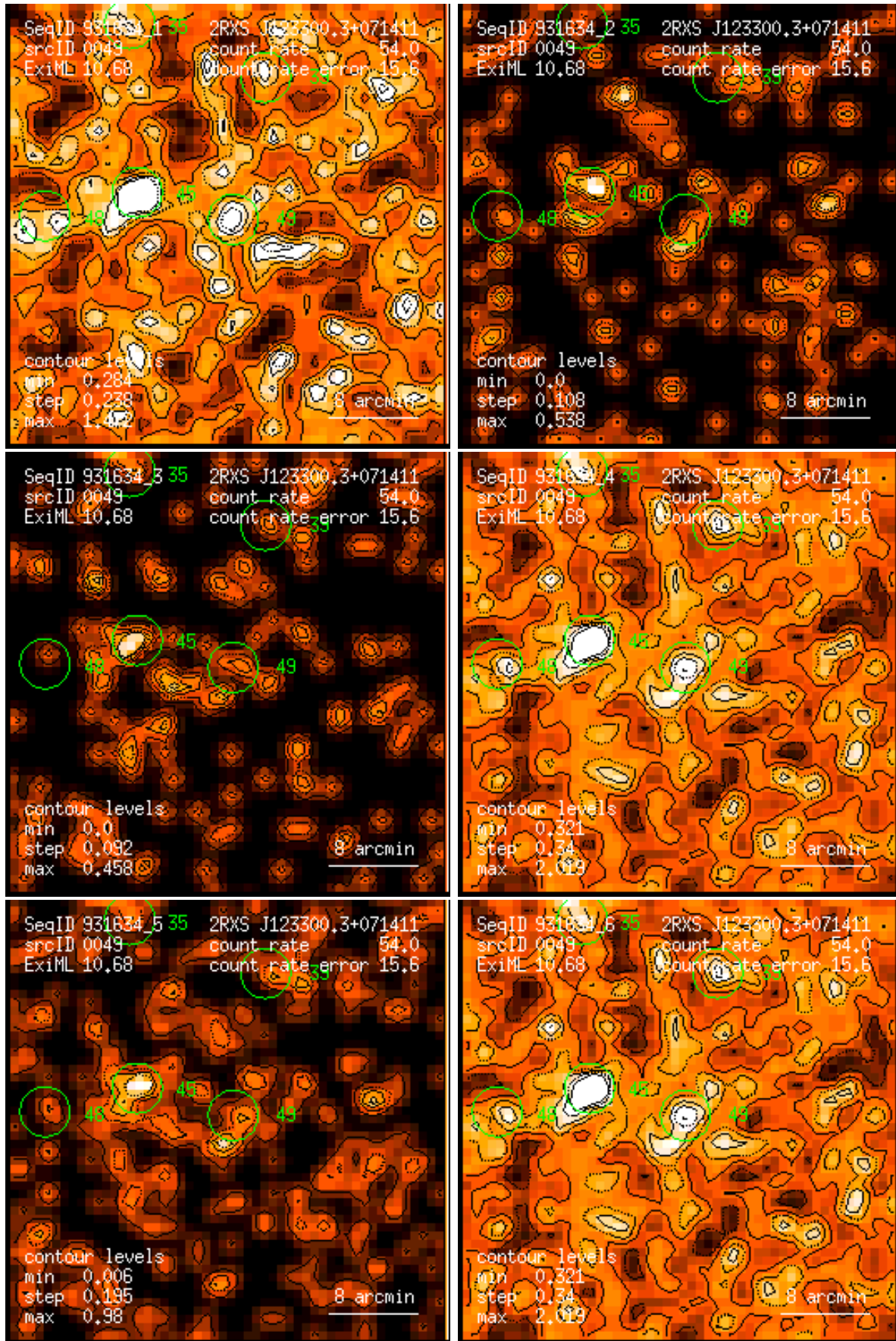
Figure 49: RASS 931634: detection 0049: band rate images, Gaussian filter: (1) PSPC channels 11 – 41, (2) 52 – 90, (3) 91 – 201, (4) 11 – 235, (5) 52 – 201, (6) 11 – 201. Broad band rates in counts/ks. Band rate contour levels in counts/ks/arcmin 2 .
