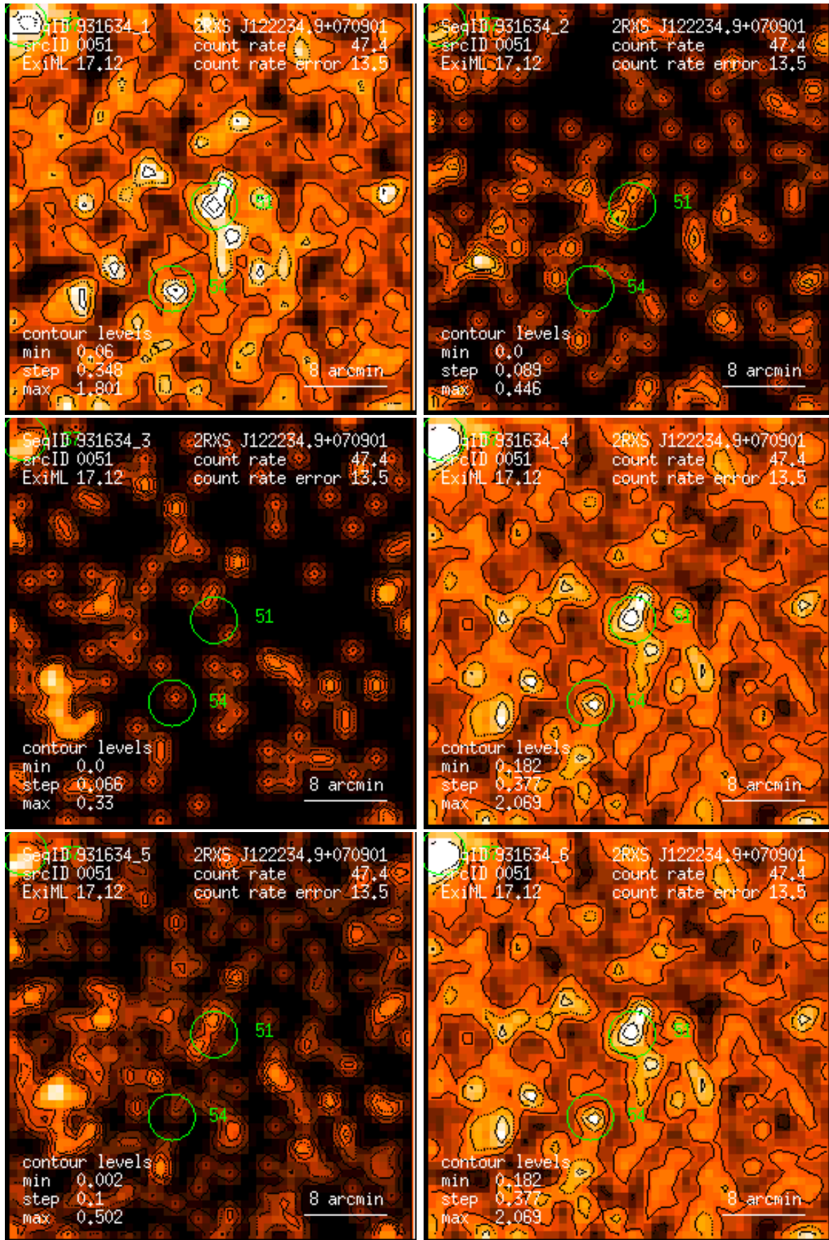
Figure 51: RASS 931634: detection 0051: band rate images, Gaussian filter: (1) PSPC channels 11 – 41, (2) 52 – 90, (3) 91 – 201, (4) 11 – 235, (5) 52 – 201, (6) 11 – 201. Broad band rates in counts/ks. Band rate contour levels in counts/ks/arcmin 2 .
