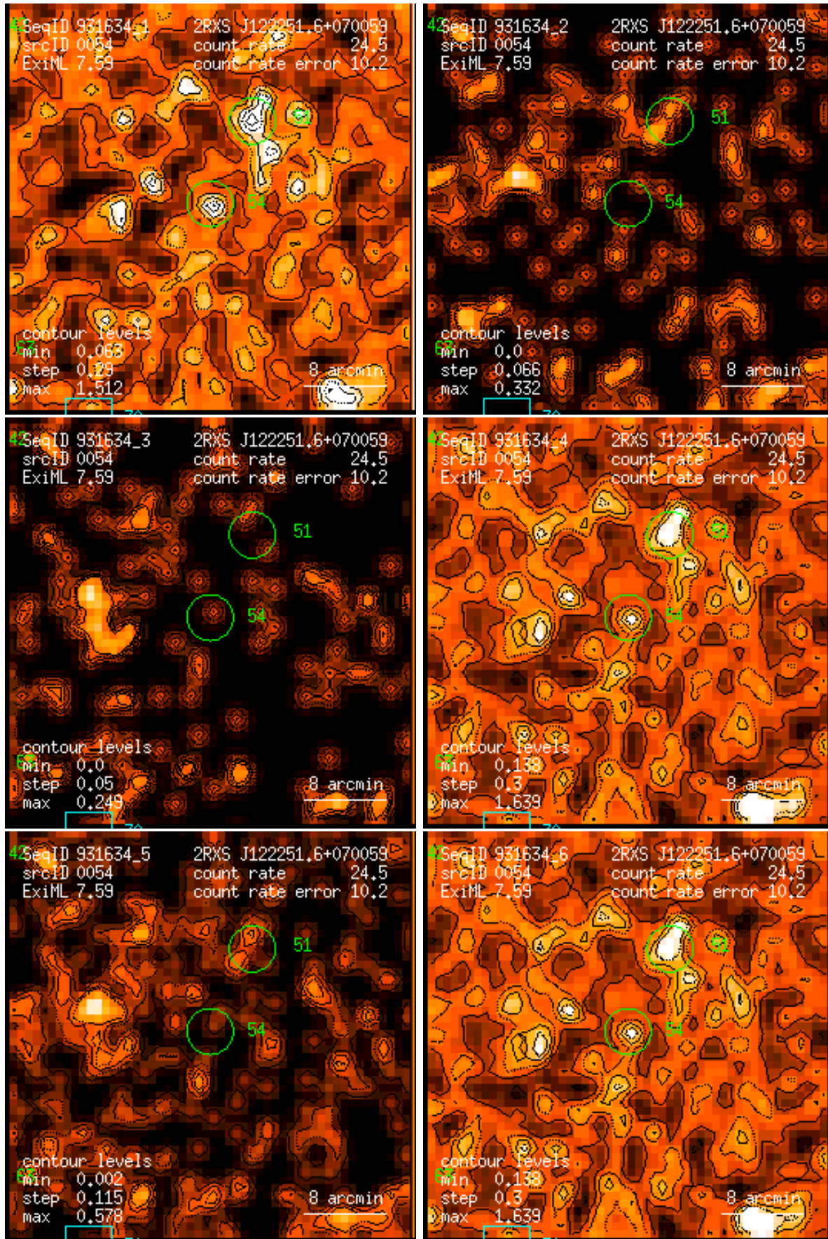
Figure 54: RASS 931634: detection 0054: band rate images, Gaussian filter: (1) PSPC channels 11 – 41, (2) 52 – 90, (3) 91 – 201, (4) 11 – 235, (5) 52 – 201, (6) 11 – 201. Broad band rates in counts/ks. Band rate contour levels in counts/ks/arcmin 2 .
