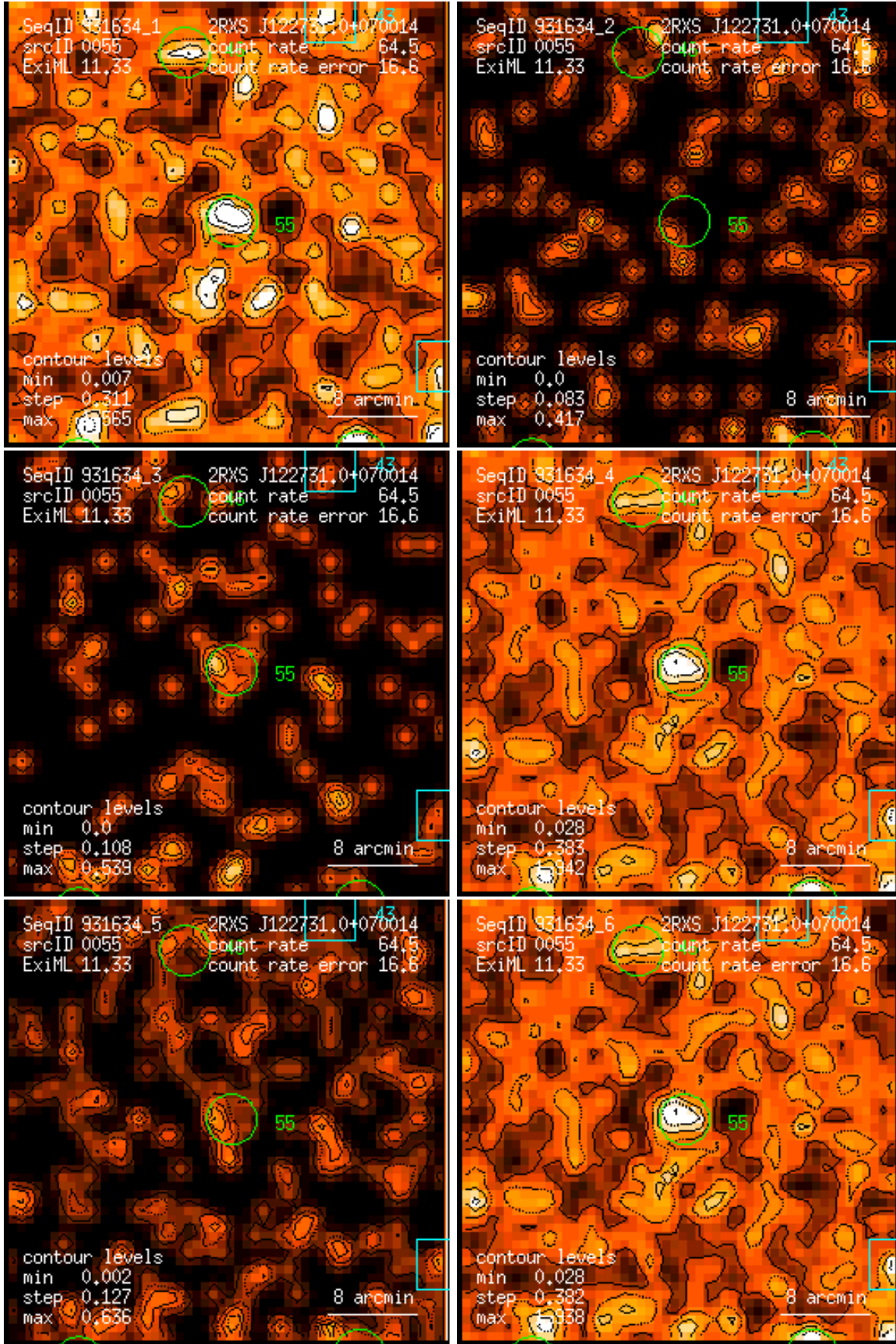
Figure 55: RASS 931634: detection 0055: band rate images, Gaussian filter: (1) PSPC channels 11 – 41, (2) 52 – 90, (3) 91 – 201, (4) 11 – 235, (5) 52 – 201, (6) 11 – 201. Broad band rates in counts/ks. Band rate contour levels in counts/ks/arcmin 2 .
