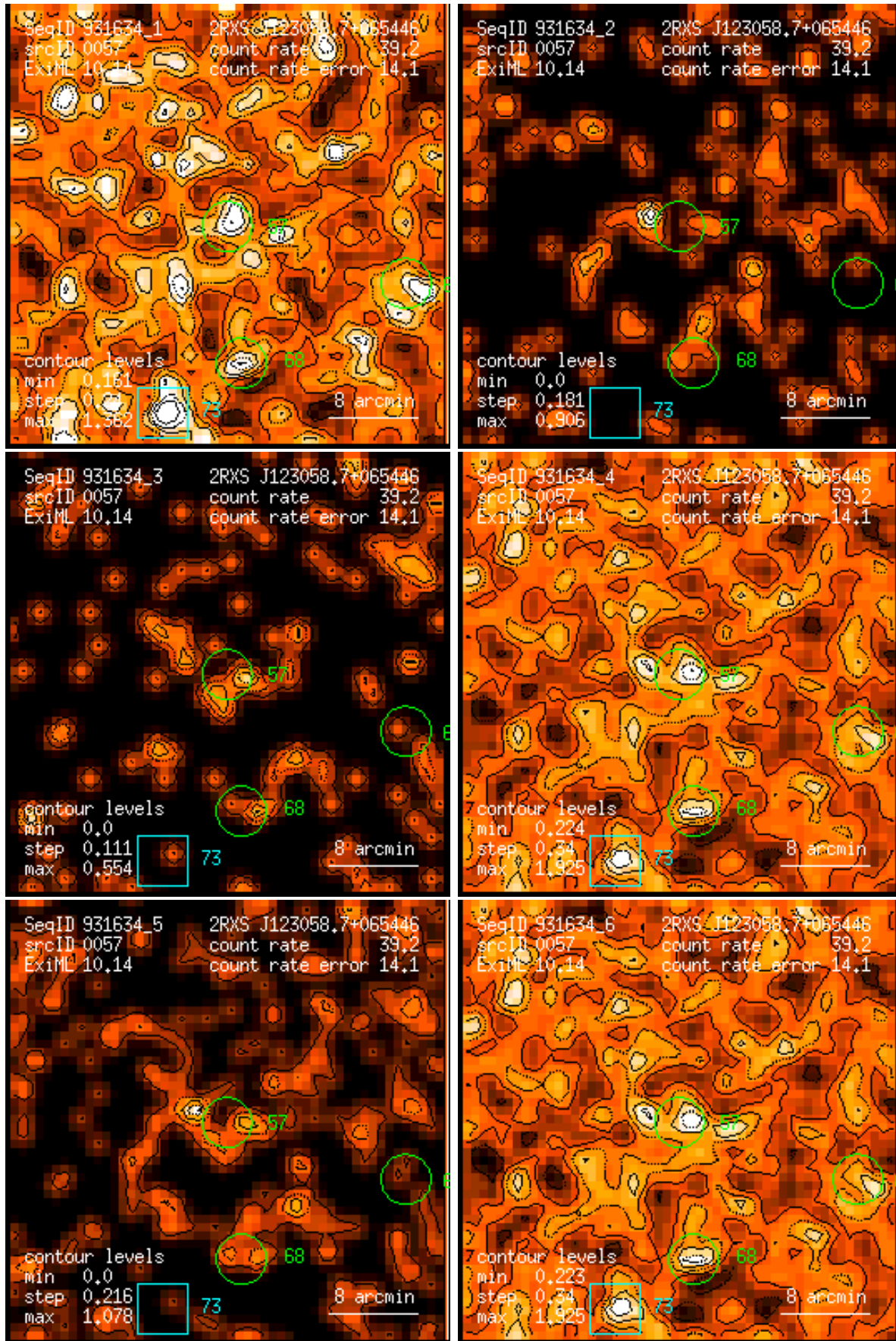
Figure 57: RASS 931634: detection 0057: band rate images, Gaussian filter: (1) PSPC channels 11 – 41, (2) 52 – 90, (3) 91 – 201, (4) 11 – 235, (5) 52 – 201, (6) 11 – 201. Broad band rates in counts/ks. Band rate contour levels in counts/ks/arcmin 2 .
