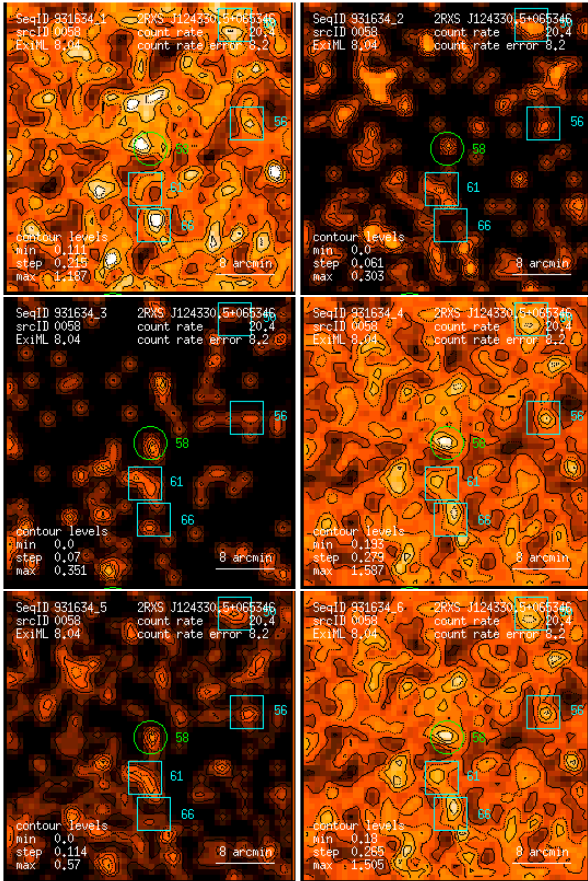
Figure 58: RASS 931634: detection 0058: band rate images, Gaussian filter: (1) PSPC channels 11 – 41, (2) 52 – 90, (3) 91 – 201, (4) 11 – 235, (5) 52 – 201, (6) 11 – 201. Broad band rates in counts/ks. Band rate contour levels in counts/ks/arcmin 2 .
