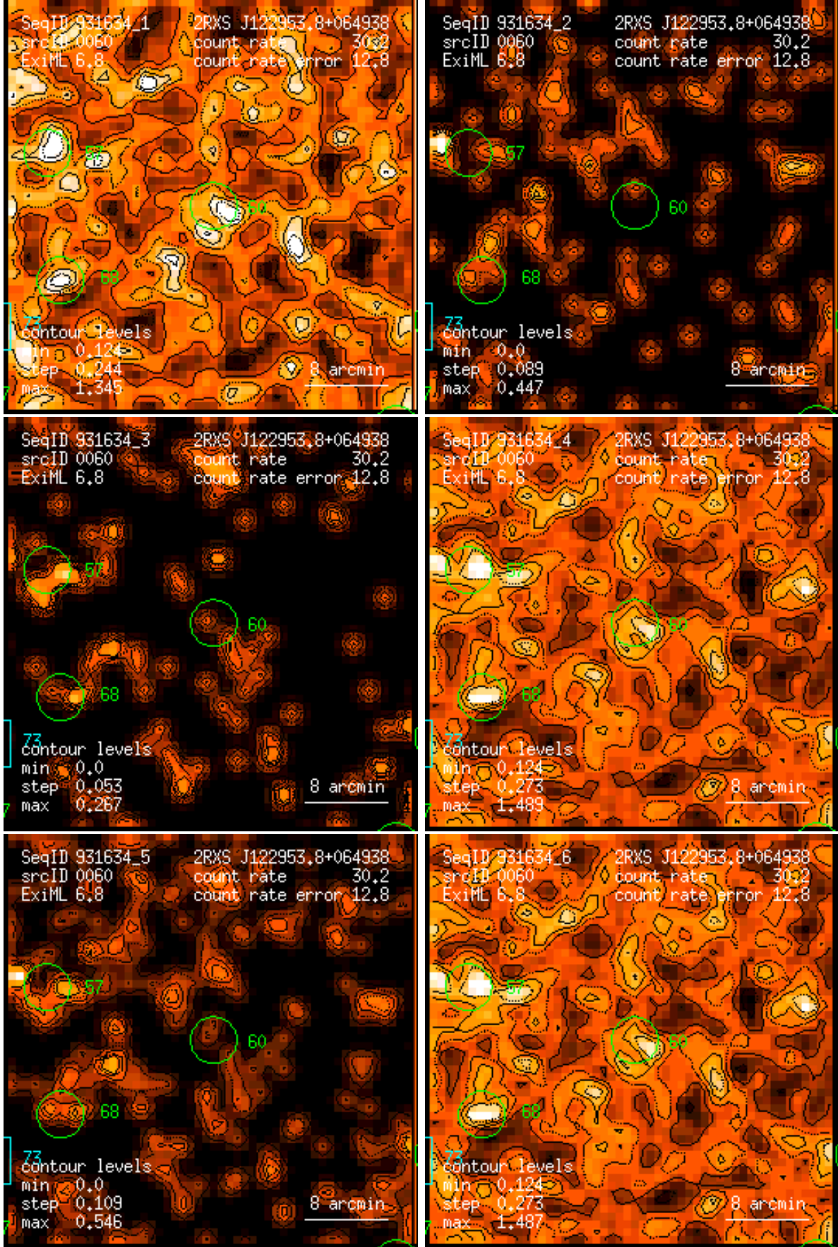
Figure 60: RASS 931634: detection 0060: band rate images, Gaussian filter: (1) PSPC channels 11 – 41, (2) 52 – 90, (3) 91 – 201, (4) 11 – 235, (5) 52 – 201, (6) 11 – 201. Broad band rates in counts/ks. Band rate contour levels in counts/ks/arcmin 2 .
