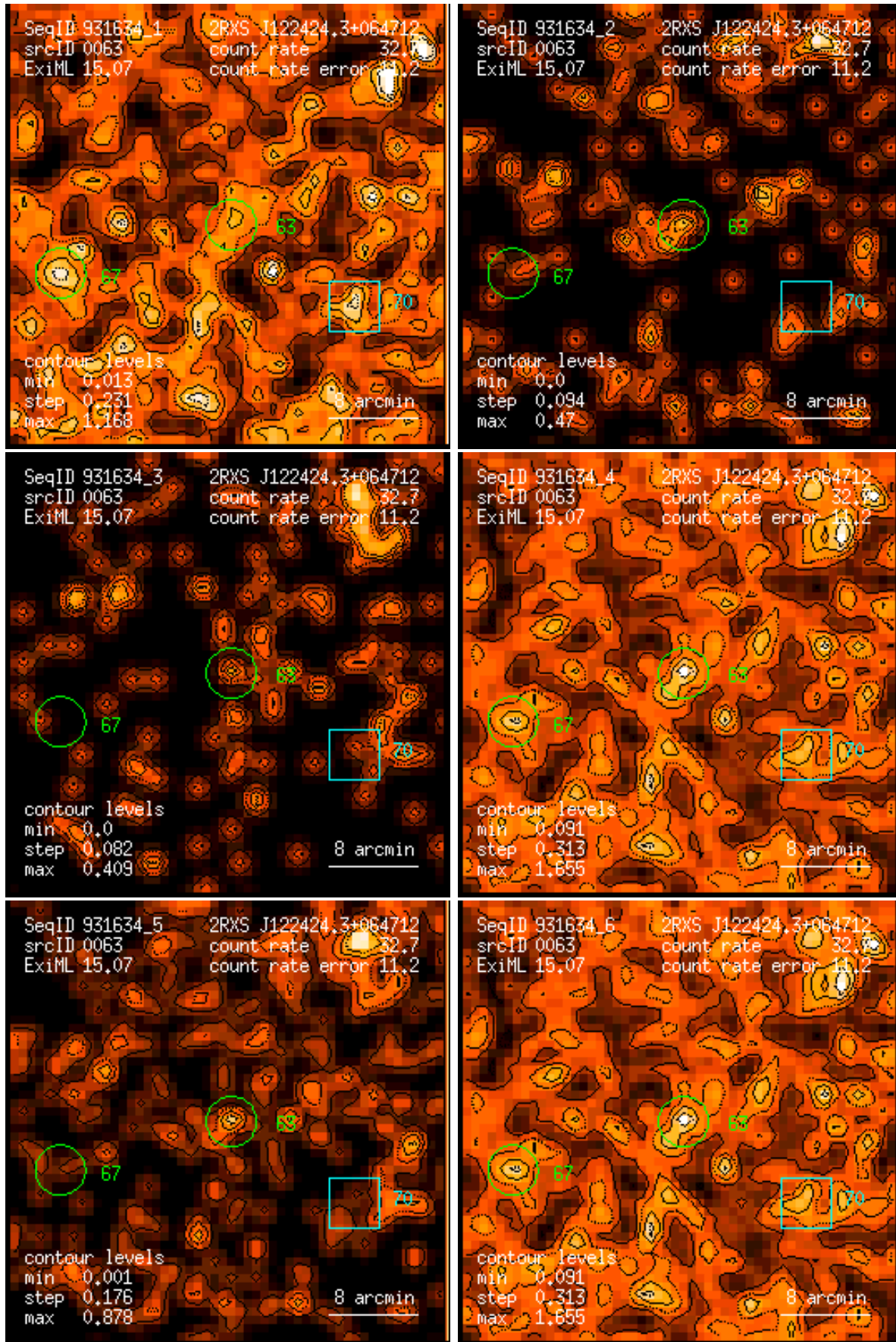
Figure 63: RASS 931634: detection 0063: band rate images, Gaussian filter: (1) PSPC channels 11 – 41, (2) 52 – 90, (3) 91 – 201, (4) 11 – 235, (5) 52 – 201, (6) 11 – 201. Broad band rates in counts/ks. Band rate contour levels in counts/ks/arcmin 2 .
