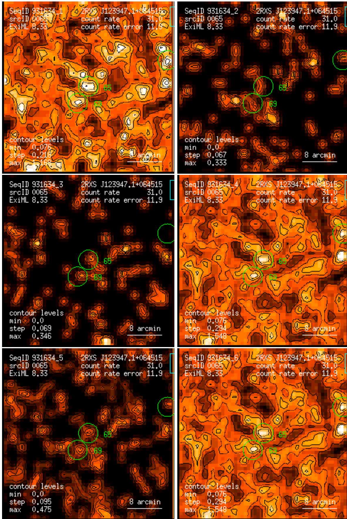
Figure 65: RASS 931634: detection 0065: band rate images, Gaussian filter: (1) PSPC channels 11 – 41, (2) 52 – 90, (3) 91 – 201, (4) 11 – 235, (5) 52 – 201, (6) 11 – 201. Broad band rates in counts/ks. Band rate contour levels in counts/ks/arcmin 2 .
