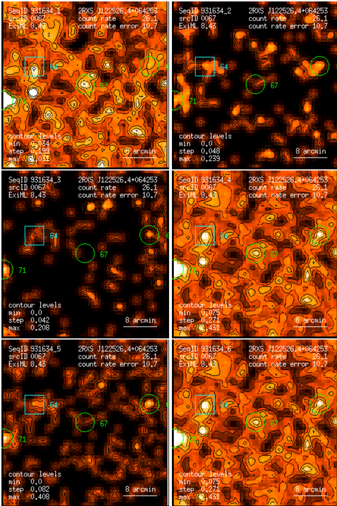
Figure 67: RASS 931634: detection 0067: band rate images, Gaussian filter: (1) PSPC channels 11 – 41, (2) 52 – 90, (3) 91 – 201, (4) 11 – 235, (5) 52 – 201, (6) 11 – 201. Broad band rates in counts/ks. Band rate contour levels in counts/ks/arcmin 2 .
