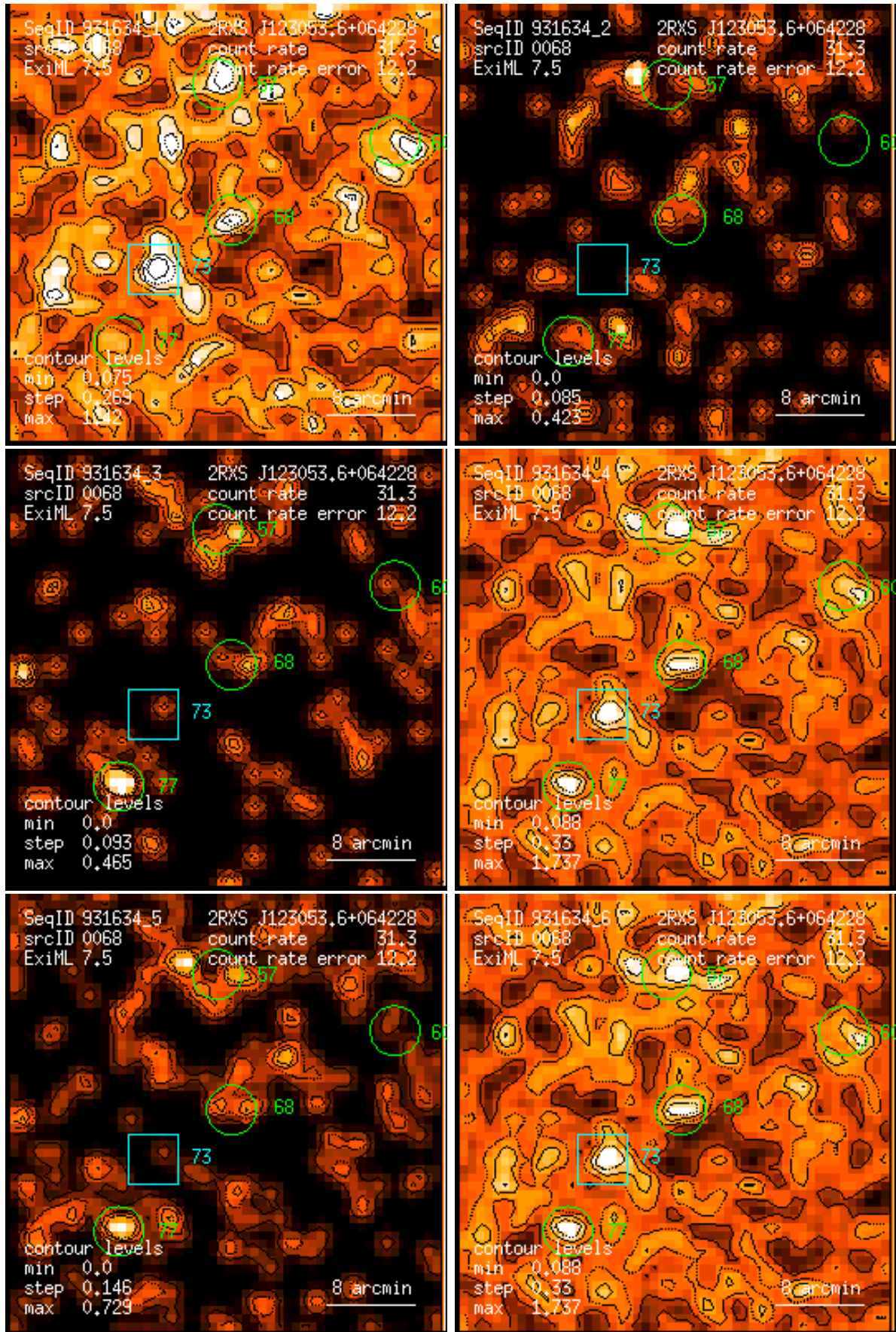
Figure 68: RASS 931634: detection 0068: band rate images, Gaussian filter: (1) PSPC channels 11 – 41, (2) 52 – 90, (3) 91 – 201, (4) 11 – 235, (5) 52 – 201, (6) 11 – 201. Broad band rates in counts/ks. Band rate contour levels in counts/ks/arcmin 2 .
